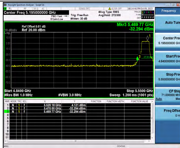
11AC40SISO_Ant1_Low_5510
