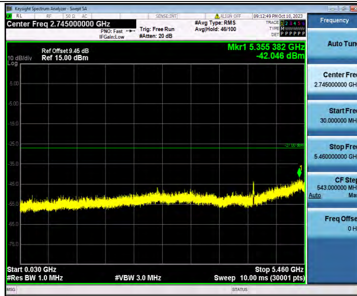
11AX20SISO_Ant1_5600_30~5460
