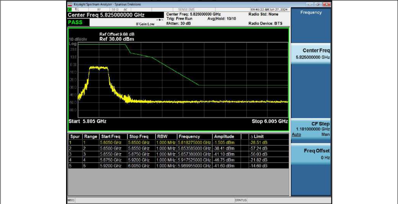
Bandedge_NVNT_ANT1_802_11ac(VHT20)_5825
