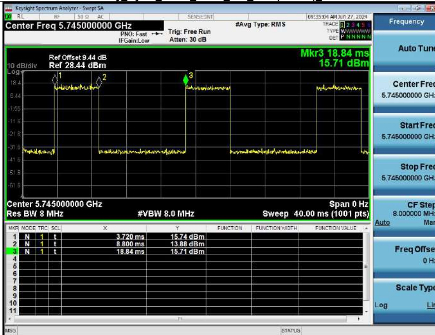
Duty_Cycle_NVNT_ANT1_802_11ac(VHT20)_5745
