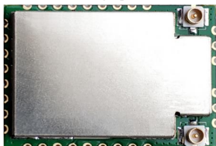
Figure 1-Top View
