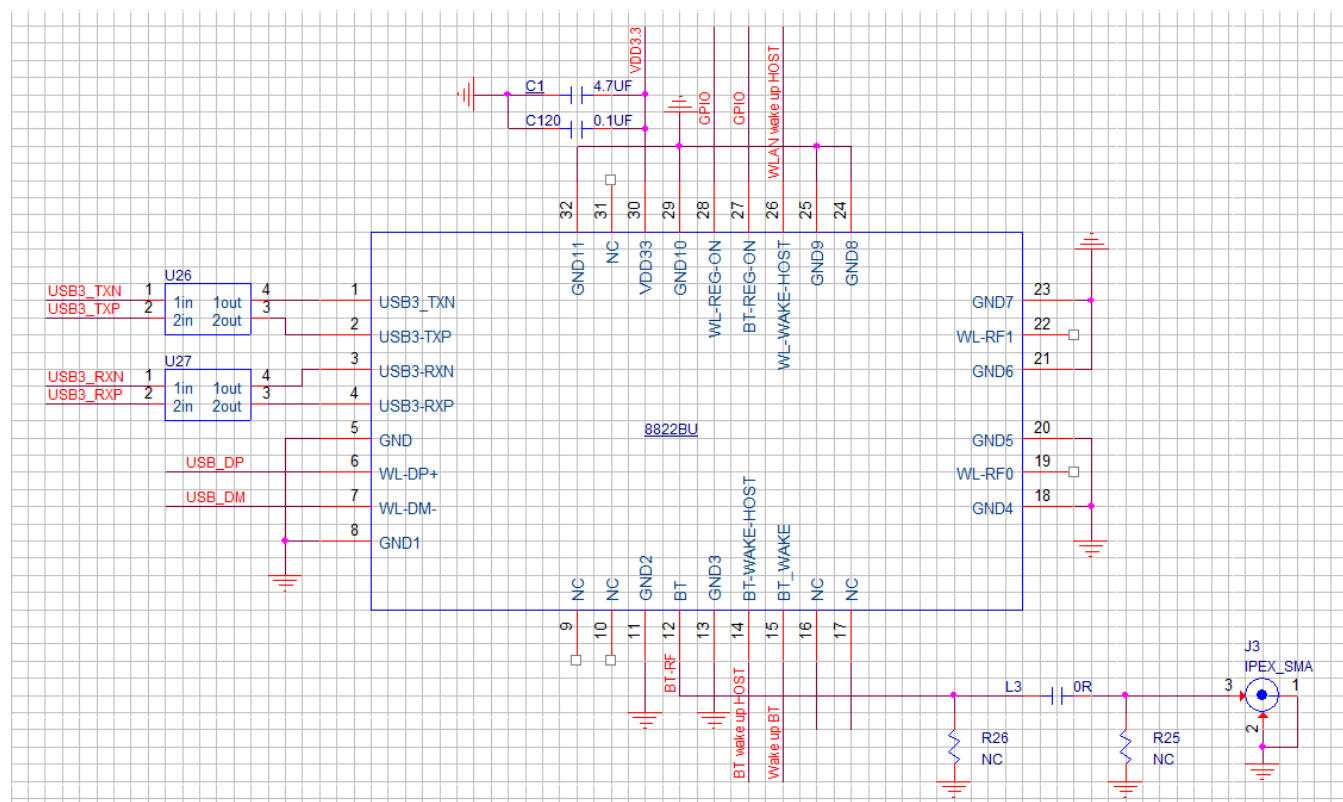
Figure 5-Typical application circuit
