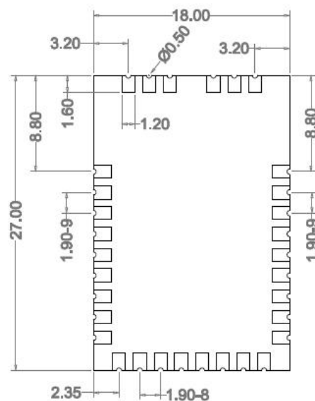
(Bottom View)
