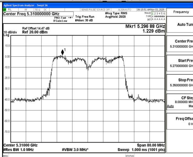
11AC40MIMO Ant2 5310
