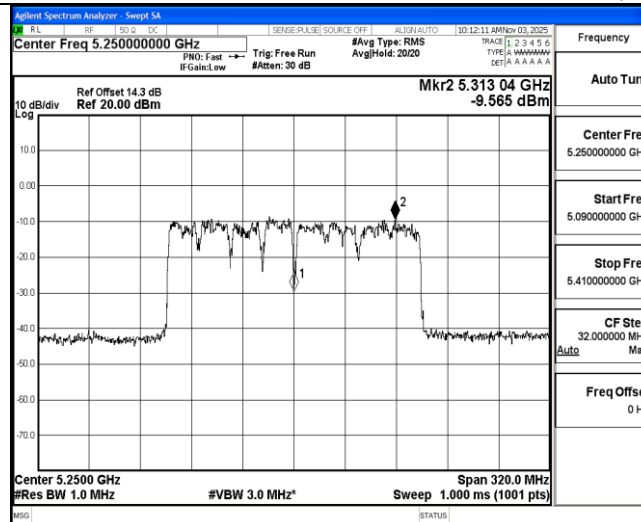
11AC160MIMO Ant2 5250 UNII-2A
