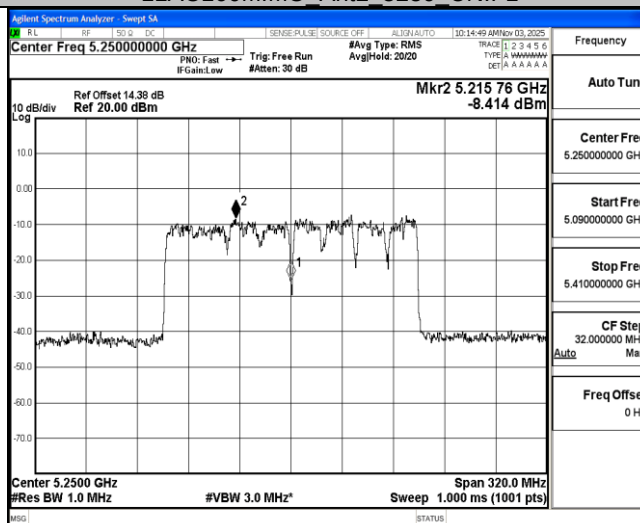
11AC160MIMO Ant1 5250 UNII-2A
