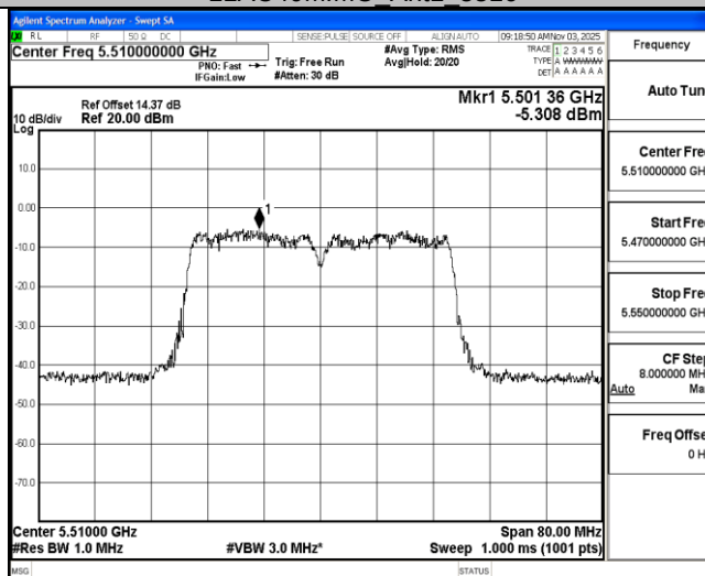
11AC40MIMO Ant2 5510
