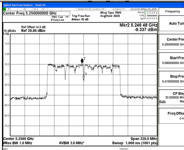
11AC160MIMO Ant2 5250 UNII-1
