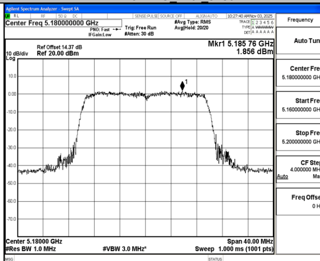
11AX20MIMO Ant2 5180
