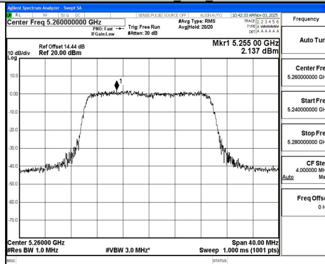
11AX20MIMO Ant2 5260
