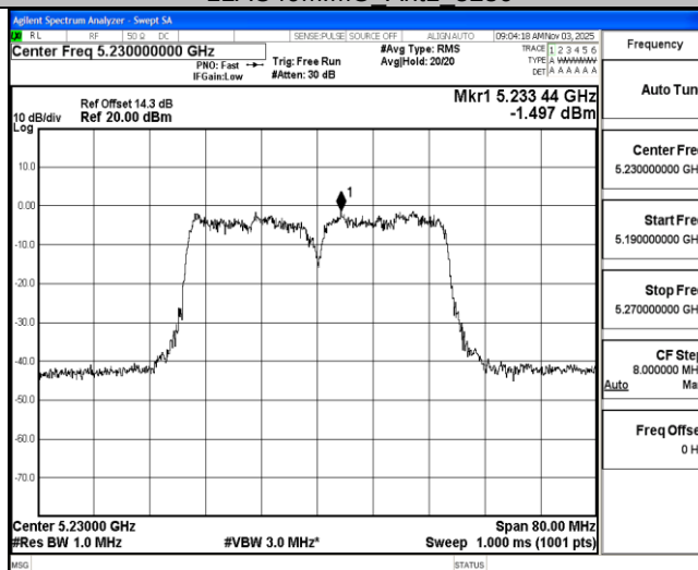
11AC40MIMO Ant2 5230
