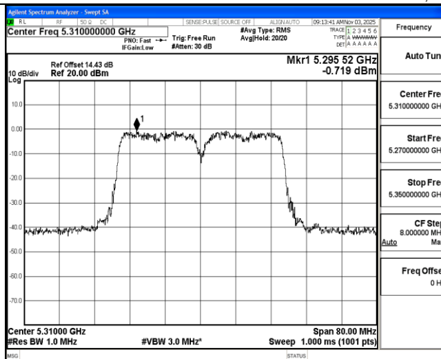
11AC40MIMO Ant2 5310
