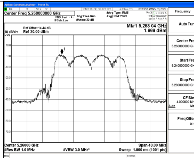
11AC20MIMO Ant2 5260
