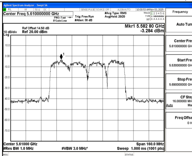
11AC80MIMO Ant2 5610
