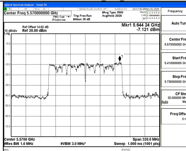
11AC160MIMO Ant2 5570
