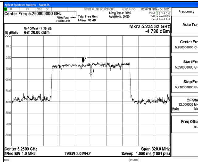
11AX160MIMO Ant1 5250 UNII-2A
