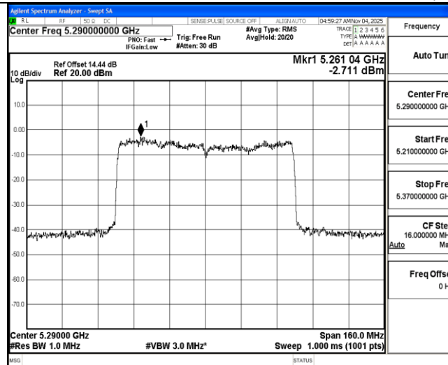
11AX80MIMO Ant2 5290
