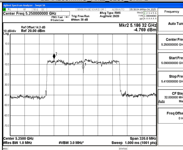
11AX160MIMO Ant2 5250 UNII-1
