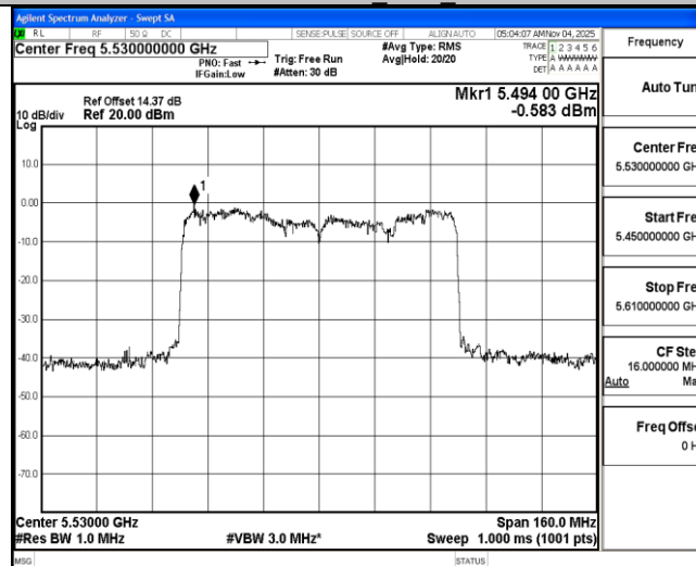
11AX80MIMO Ant2 5530
