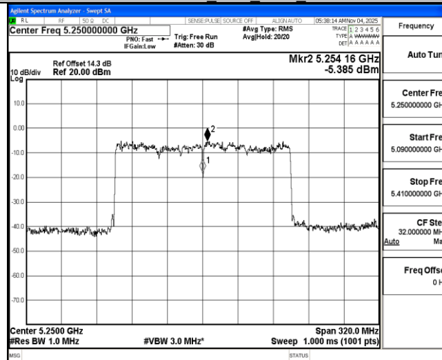
11AX160MIMO Ant2 5250 UNII-2A
