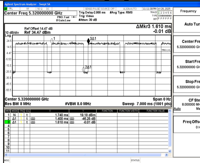
11N20MIMO Ant2 5320
