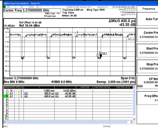
11N40MIMO Ant2 5270
