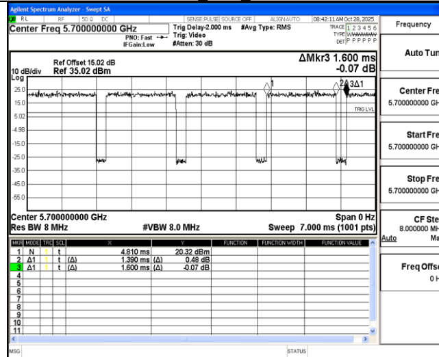
11A Ant2 5700
