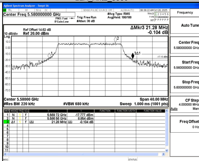
11A Ant2 5580
