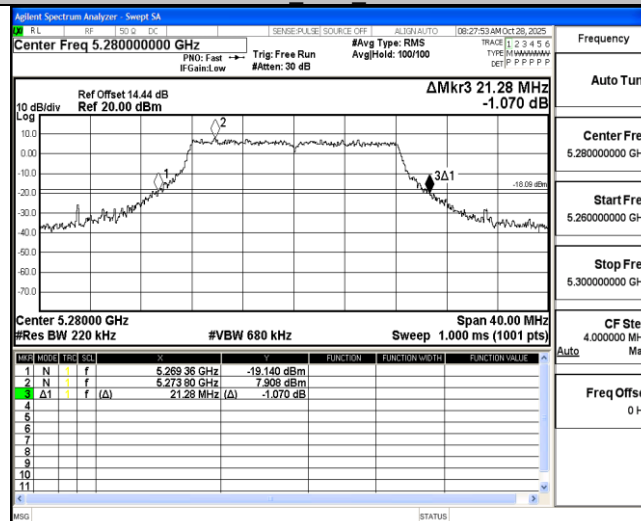
11A Ant2 5280
