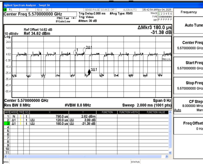
11AX160MIMO Ant2 5570
