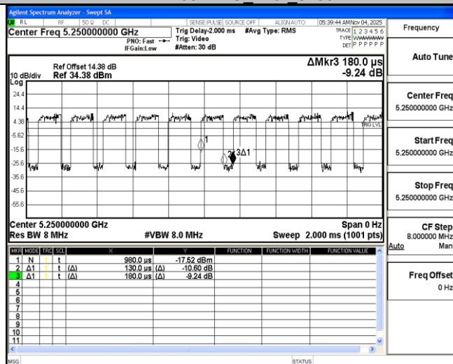
11AX160MIMO Ant2 5250
