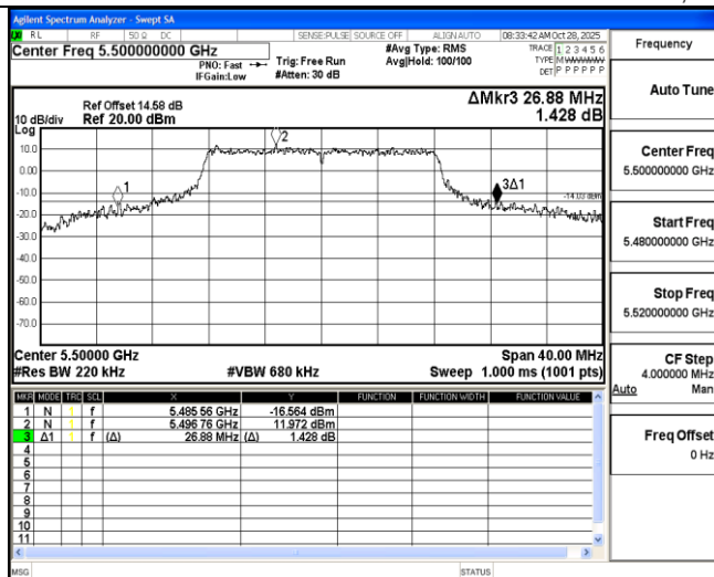
11A Ant2 5500
