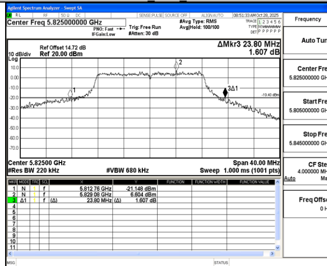
11A Ant2 5825
