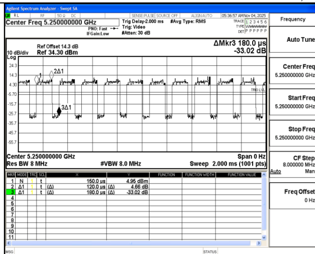
11AX160MIMO Ant2 5250
