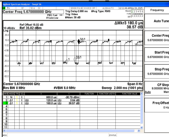
11AX40MIMO Ant2 5670
