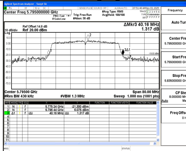
11N40MIMO Ant2 5795
