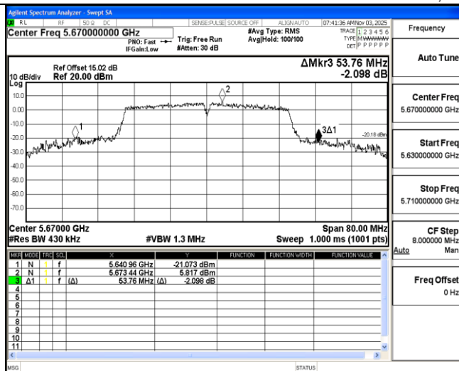
11N40MIMO Ant2 5670
