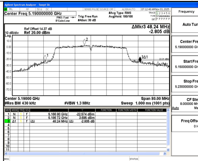
11N40MIMO Ant2 5190
