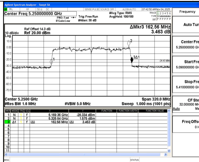
11AX160MIMO Ant2 5250
