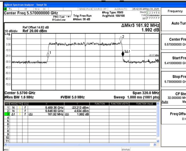
11AX160MIMO Ant2 5570
