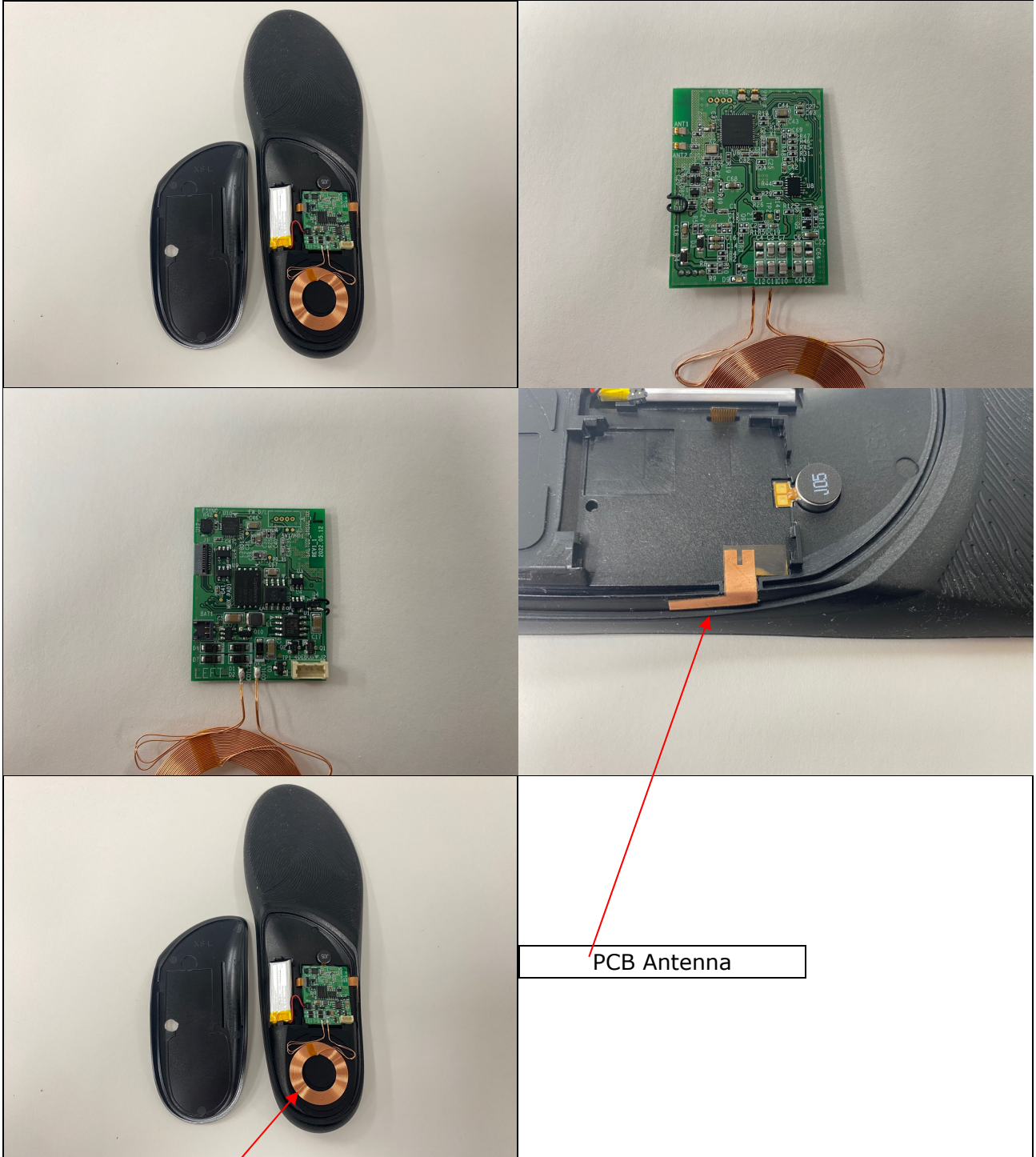
wireless charging Antenna (RX only)
