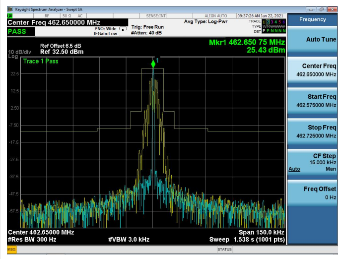
Channel 19: 462.6500MHz
