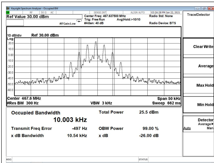
Channel 11: 467.6375MHz
