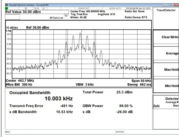
Channel 19: 462.6500MHz
