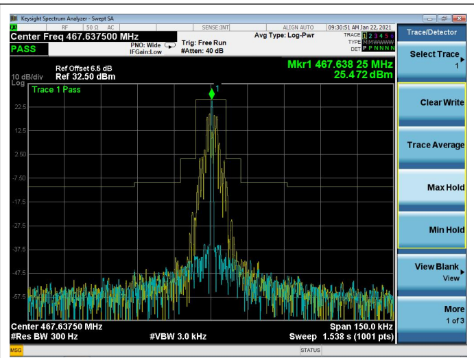
Channel 11: 467.6375MHz
