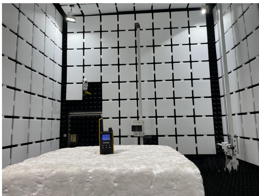
Above 1GHz- Radiated Emissions Measurement
