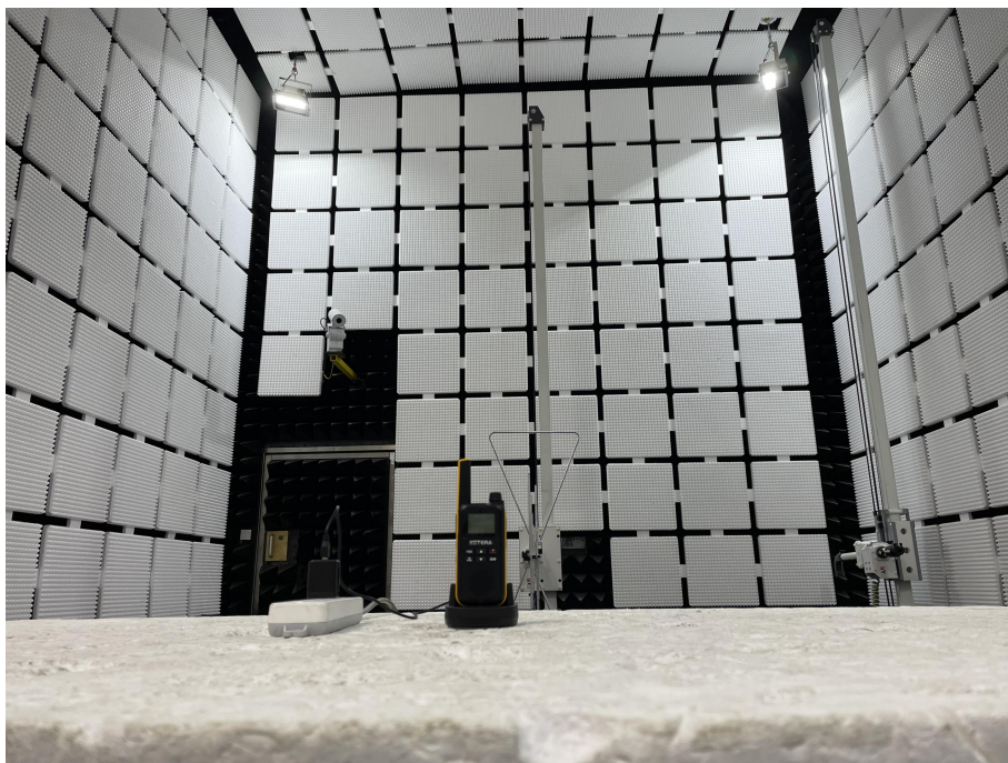
Below 1GHz- Radiated Emissions Measurement
