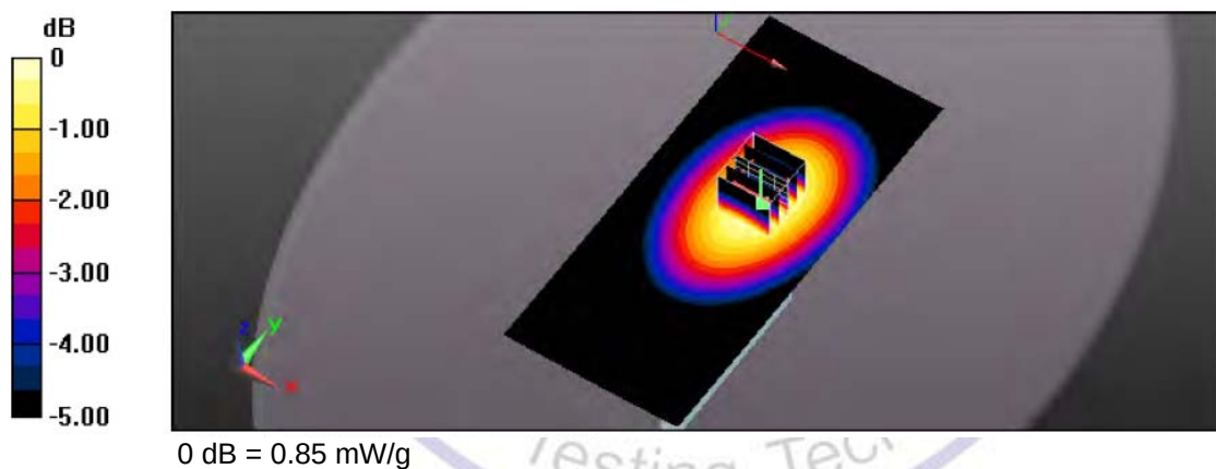
Figure 2: Face held for FM Modulation at 12.5KHz Channel Separation Front towards Phantom 467.6375 MHz
