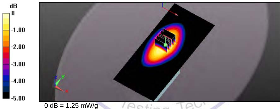
Figure 3: Body-worn for FM Modulation at 12.5KHz Channel Separation; Front towards Ground 462.6500 MHz
