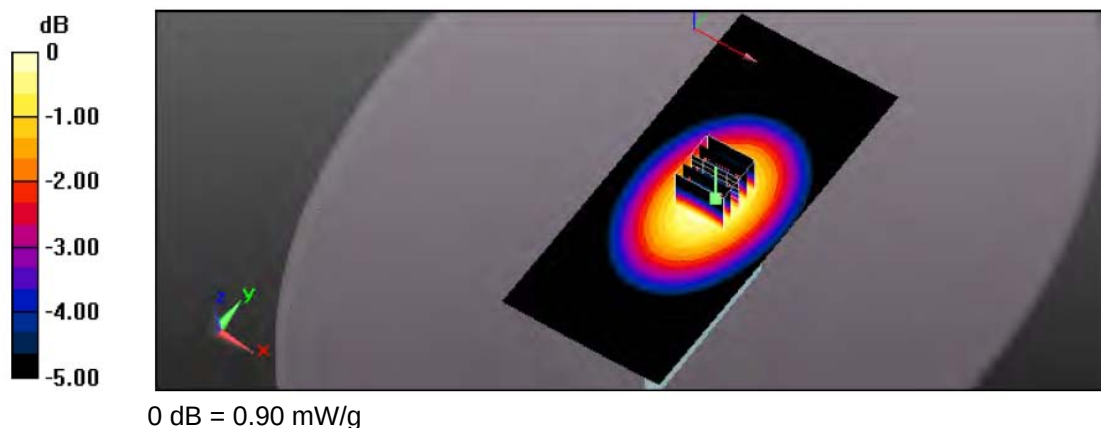
Figure 1: Face held for FM Modulation at 12.5KHz Channel Separation Front towards Phantom 462.6500 MHz
