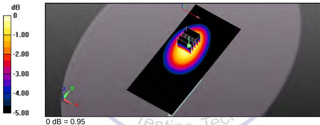
Figure 4: Body-worn for FM Modulation at 12.5KHz Channel Separation; Front towards Ground 467.6375 MHz
