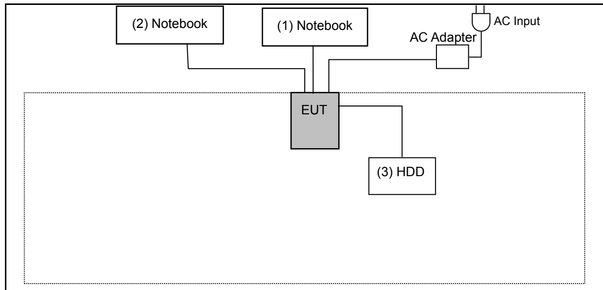
Conducted Emission
