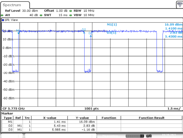
802.11ax-80 MHz
