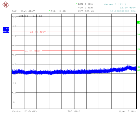
Figure 8.6-16: Radiated spurious emissions 18-25 GHz on low channel
