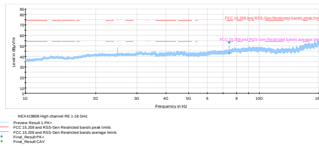
Figure 8.6-15: Radiated spurious emissions 1-18 GHz on high channel
