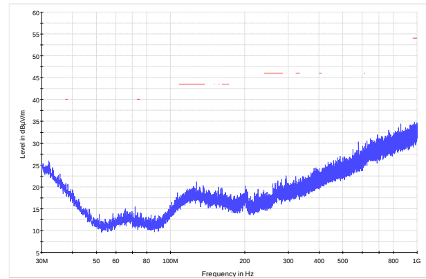
NEX419806 Mid channel RE PK+, MAXH FCC 15.209 and RSS-Gen Restricted bands average limits
