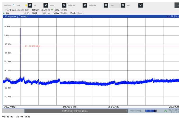
Figure 8.6-9: Conducted spurious emissions on high channel
