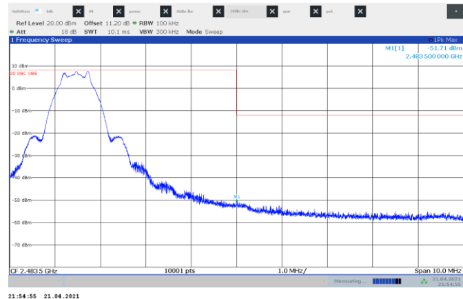
Figure 8.6-2: Conducted Band edge spurious emissions at 2483.5 MHz
