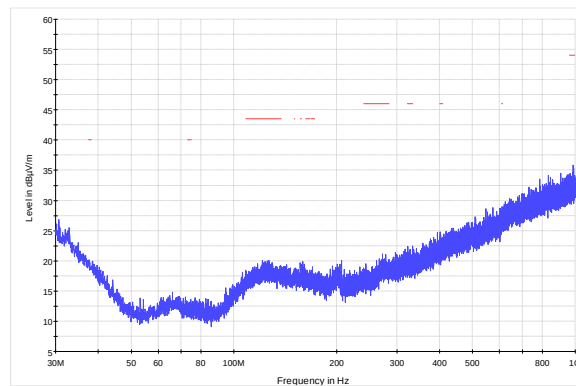
NEX419806 high channel RE PK+, MAXH FCC 15.209 and RSS-Gen Restricted bands average limits
