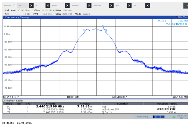
Figure 8.4-2: 6 dB bandwidth on mid channel
