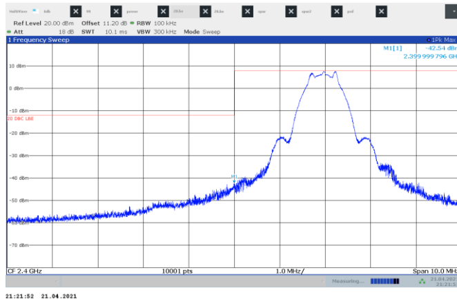
Figure 8.6-1: Conducted Band edge spurious emissions at 2400 MHz
