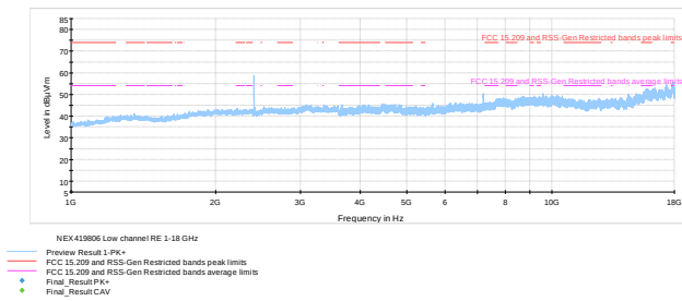
Figure 8.6-13: Radiated spurious emissions 1-18 GHz on low channel
