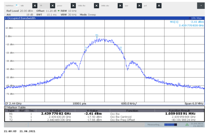
Figure 8.4-5: 99% occupied bandwidth on mid channel
