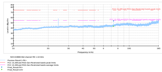
Figure 8.6-14: Radiated spurious emissions 1-18 GHz on mid channel
