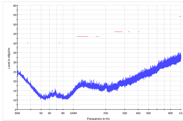
NEX419806 Low channel RE PK+, MAXH FCC 15.209 and RSS-Gen Restricted bands average limits
