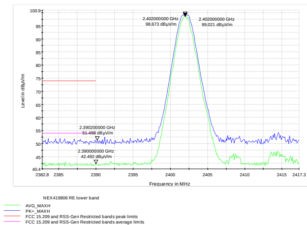
Figure 8.6-3: Radiated Restricted band edge spurious emissions low ch. -
