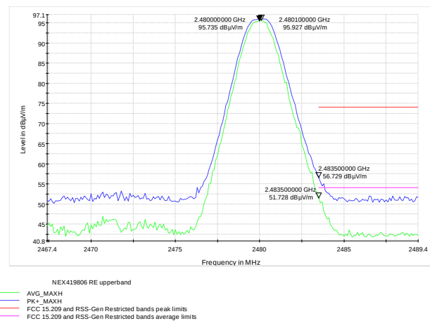
Figure 8.6-4: Radiated Restricted band edge spurious emissions high ch
