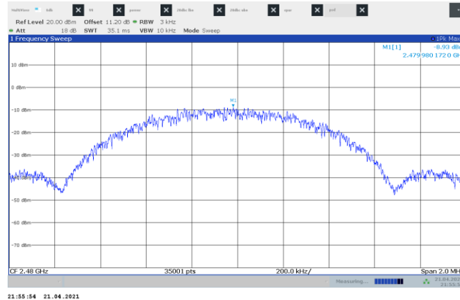
Figure 8.7-3: PSD on high channel
