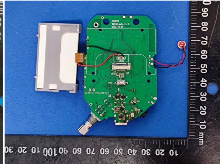
FM Antenna
