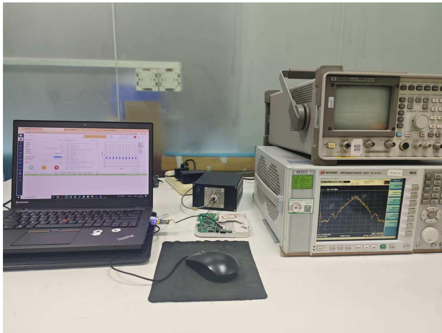
RF Performance Test
