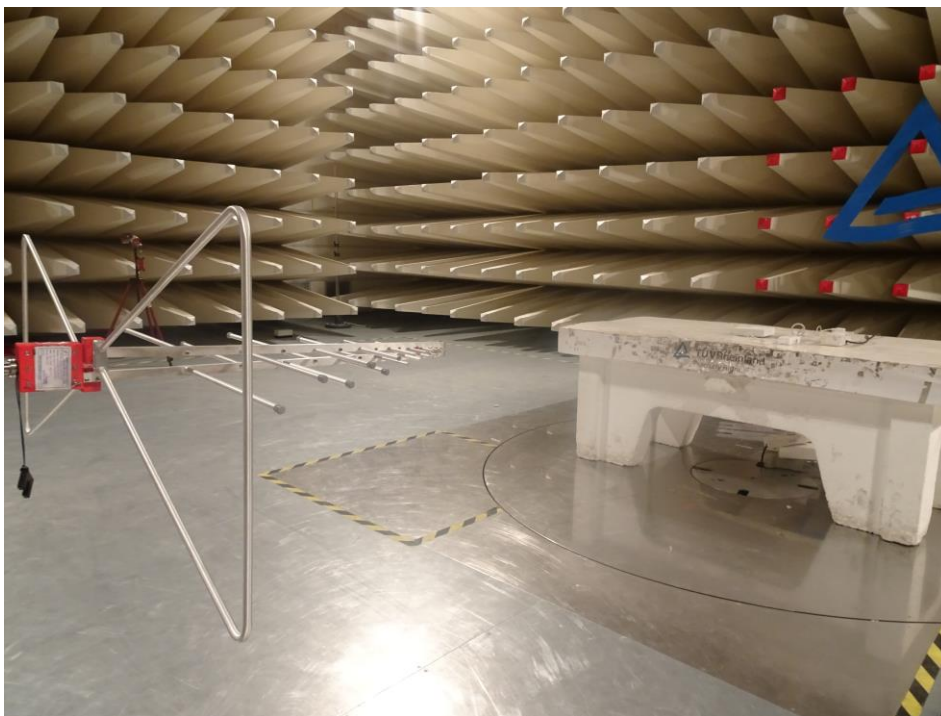
Test Setup
