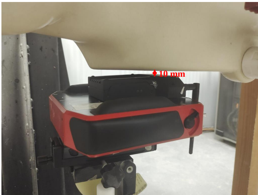
Body Back With Antenna Fold Setup Photo (10mm)
