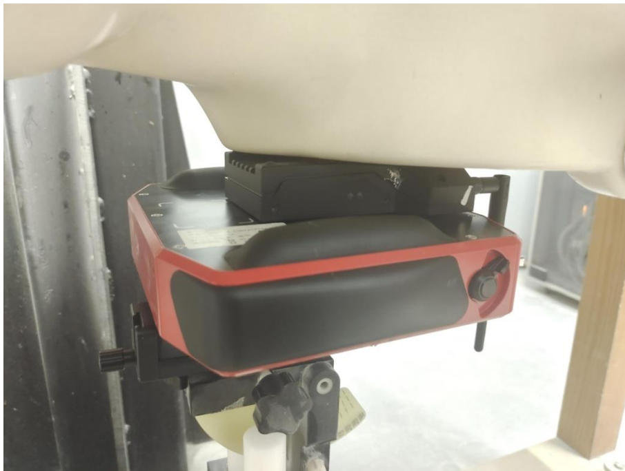
Handheld With Antenna Fold Setup Photo (0mm)
