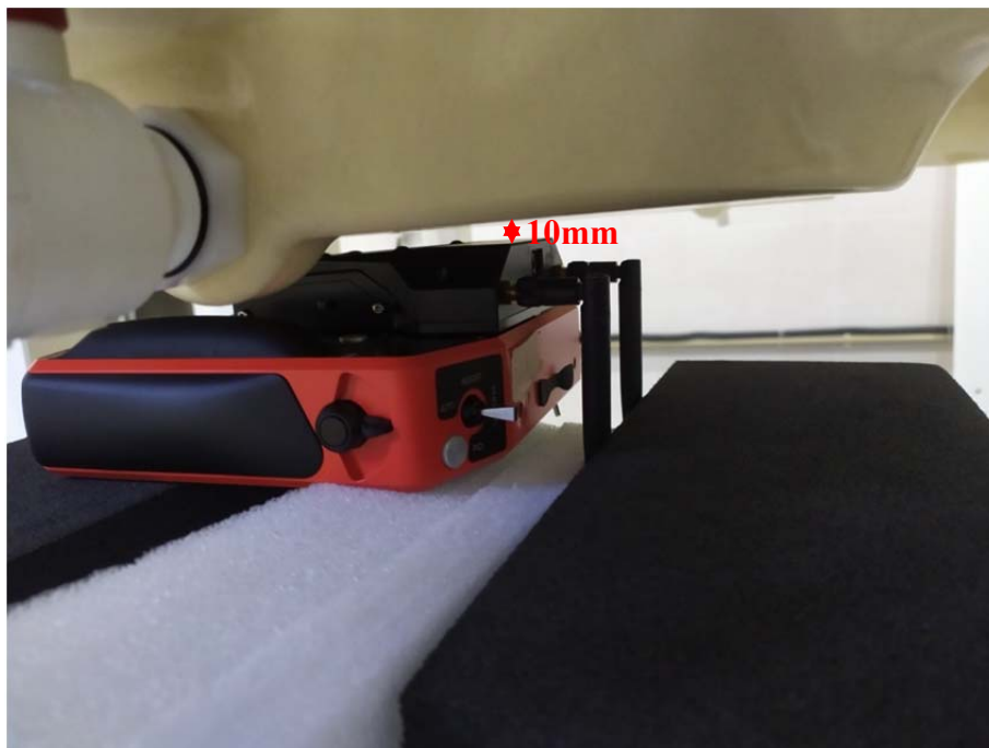
Close to Body Back With Antenna Fold Setup Photo(10mm)
