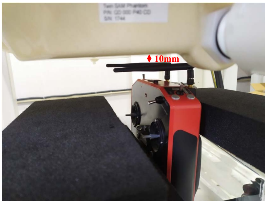
Close to Body Top Setup Photo(10mm)
