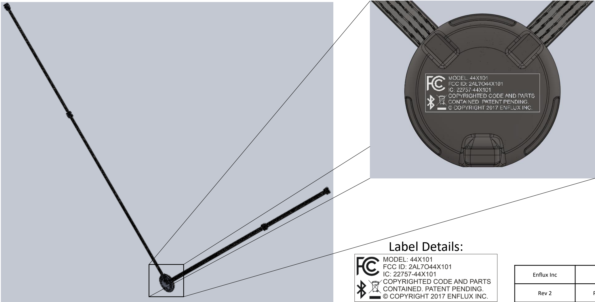
Back of Module Case
