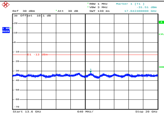
13.6GHz–20GHz
