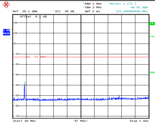
30 MHz–1GHz
