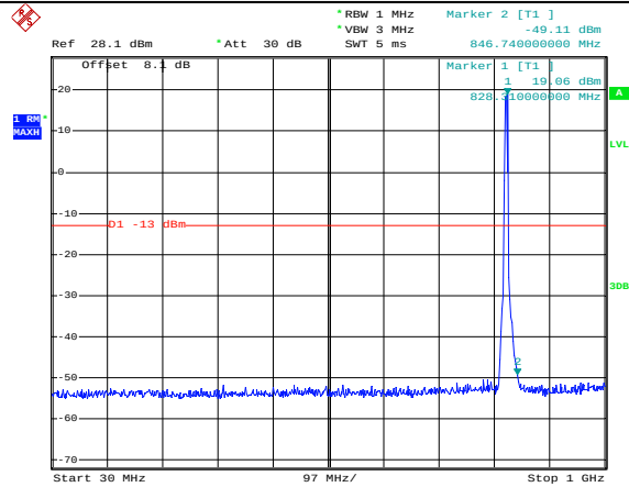
Channel 4132 / 826.4 MHz
