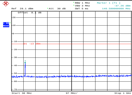
30 MHz–1GHz
