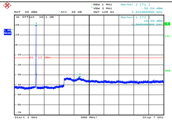
1GHz–7GHz
