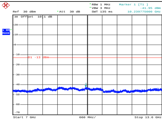
7GHz–13.6GHz
