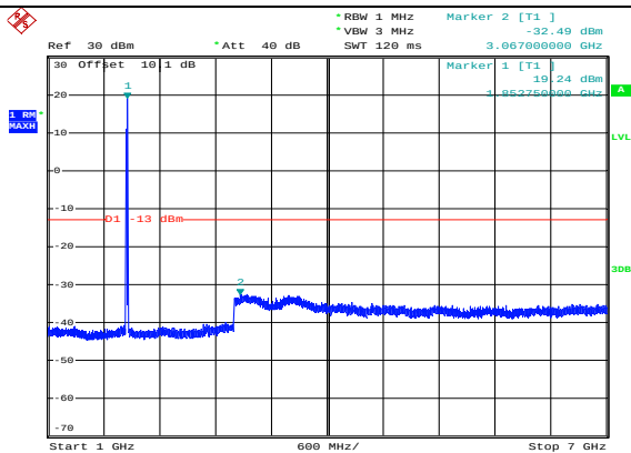
1GHz–7GHz
