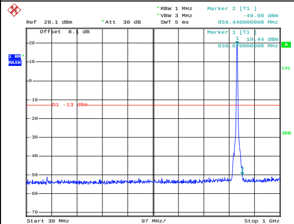
Channel 4183 / 836.6 MHz
