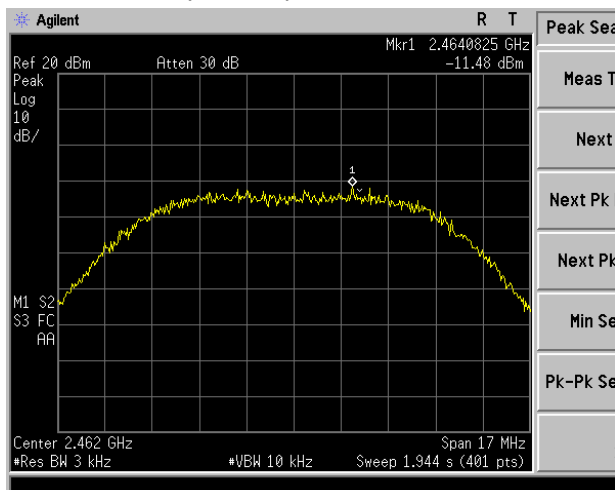
(802.11b) channel 11
