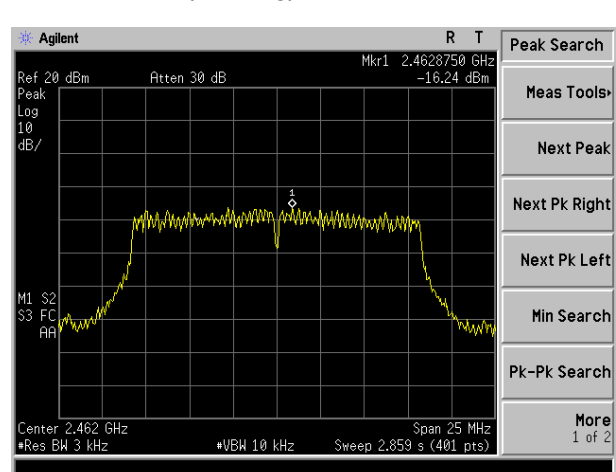
(802.11g) channel 11
