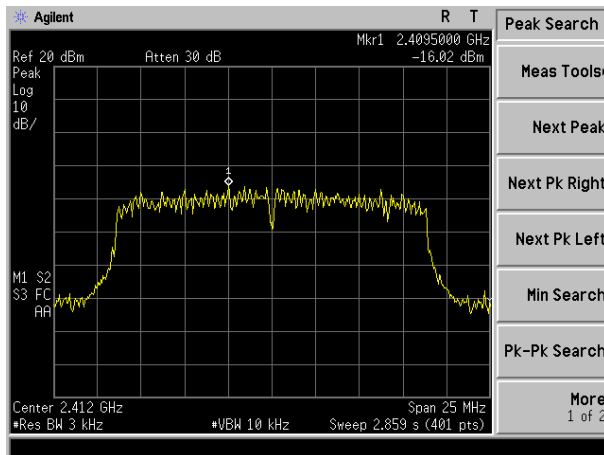
(802.11n20) channel 1
