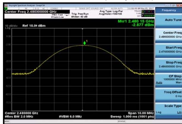
BT DH5 CH78, Carrier frequency (MHz): 2480
