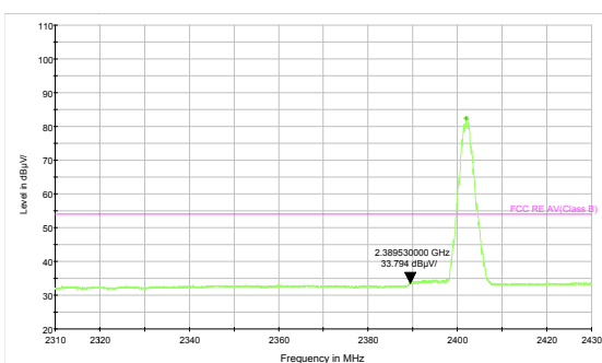
3DH5-Channel 0: Average
