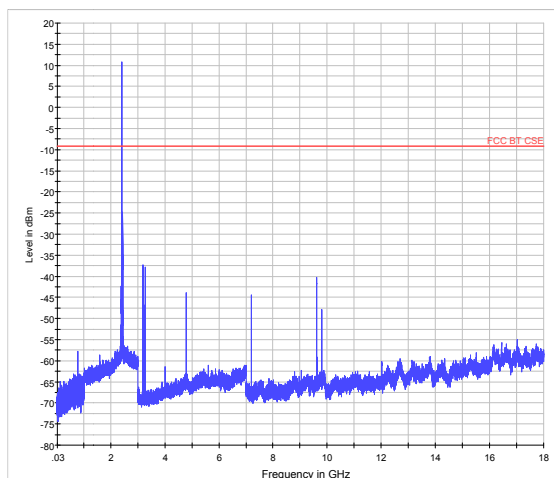
GFSK-CH0 30MHz to 18GHz
