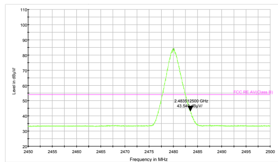
3DH5-Channel 78: Peak
