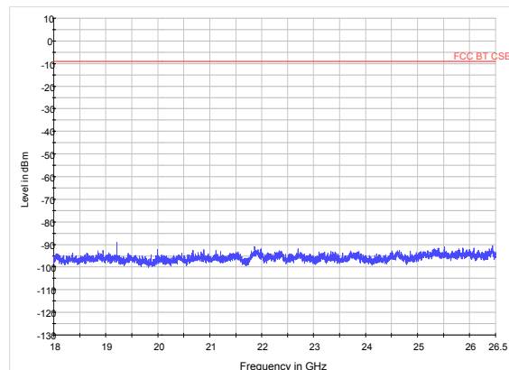
GFSK-CH0 18GHz to 26.5GHz
