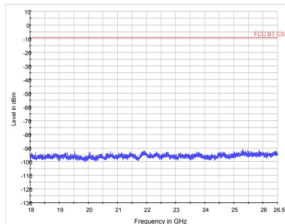
GFSK- CH39 18GHz to 26.5GHz
