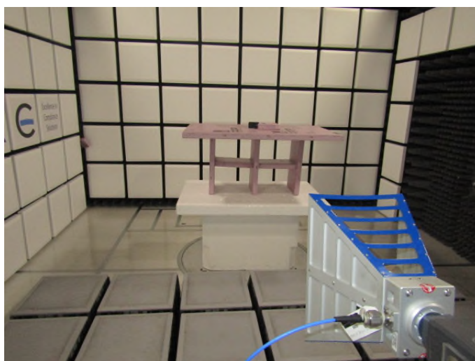
Figure 3: Radiated Emissions – Above 1GHz – Front View
