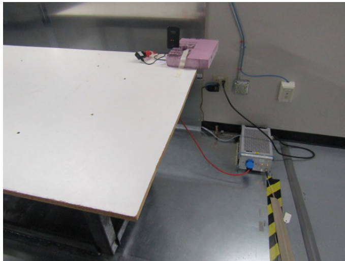
Figure 4: Power Line Conducted Emissions – Front View
