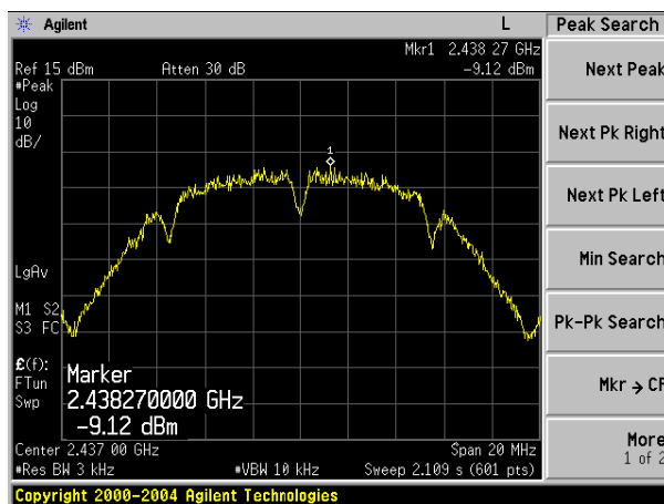
(802.11b) channel 6
