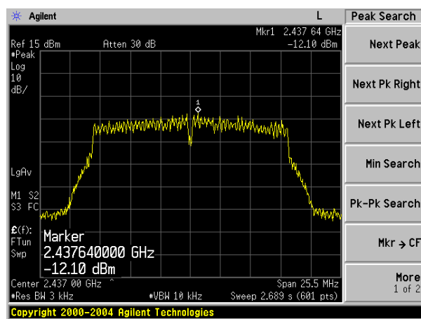
(802.11g) channel 6
