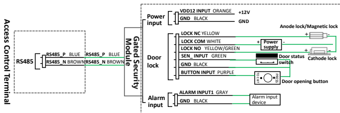
Figure 3-2 Wiring Schematic Diagrams (with Security Module)
