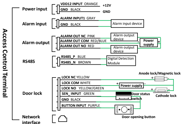
Figure 3-1 Wiring Schematic Diagrams (without Security Module)
