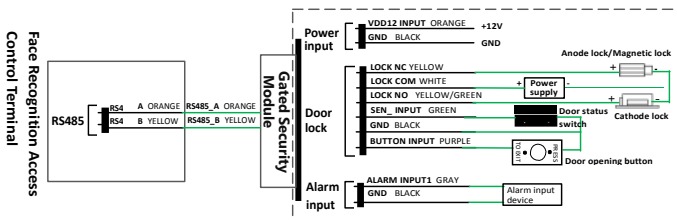
Figure 3-2 Wiring Schematic Diagrams (with Security Module)
