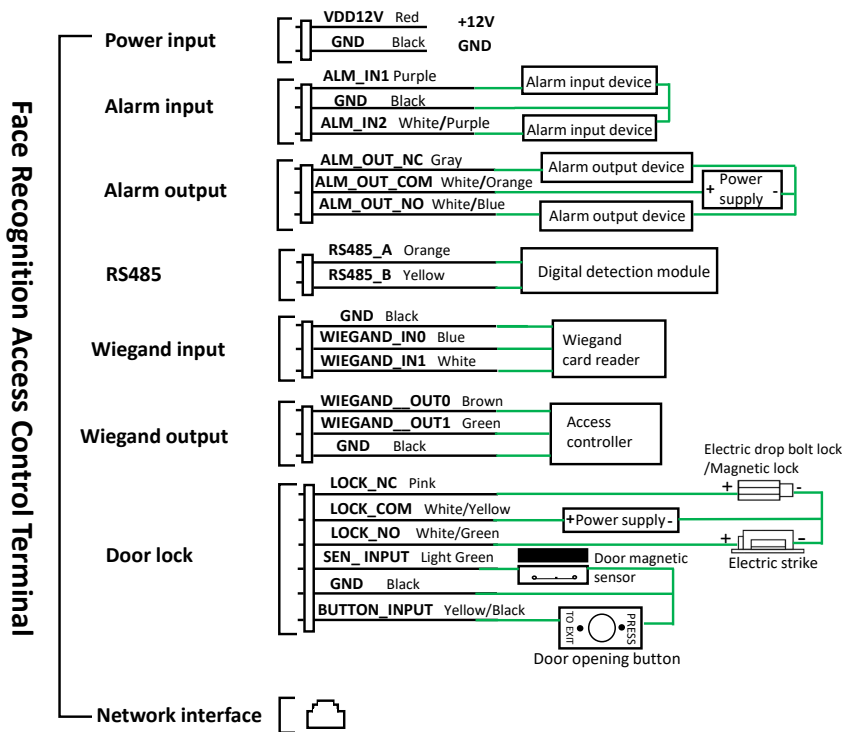
Figure 3-1 Wiring Schematic Diagrams (without Security Module)
