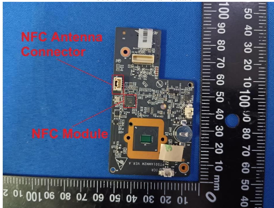
RF Module & Antenna Location-2
