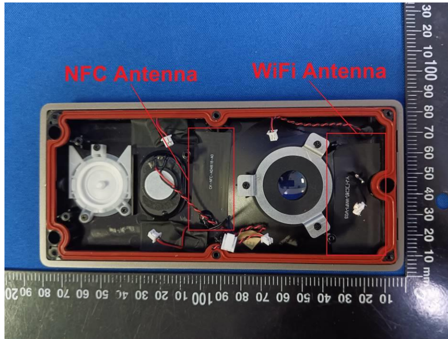
RF Module & Antenna Location-3
