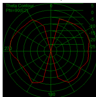
Efficiency: 55.6 %
