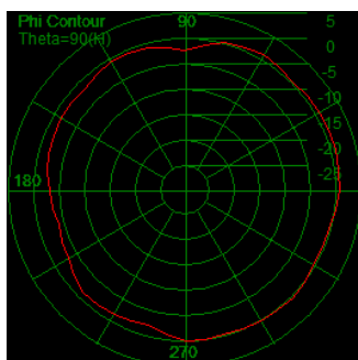
Peak Gain: 2.77dBi
