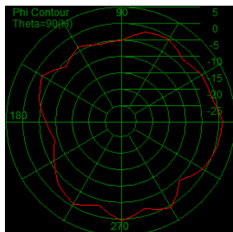
Peak Gain: 3.17dBi
