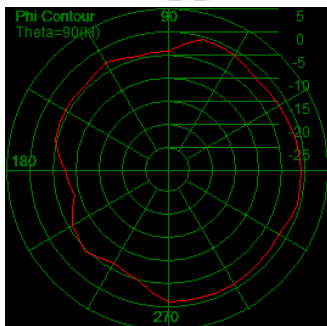
Peak Gain:3.15dBi
