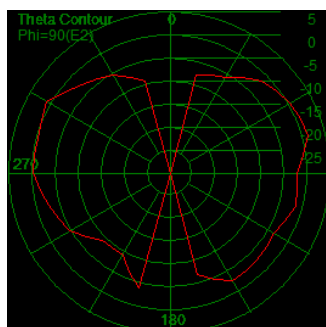
Efficiency: 64.7%
