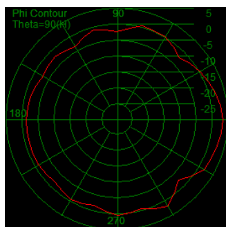
Peak Gain: 3.06 dBi
