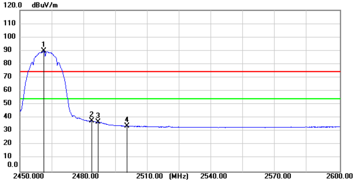
11b_TX_CH_11_Vertical_Average
