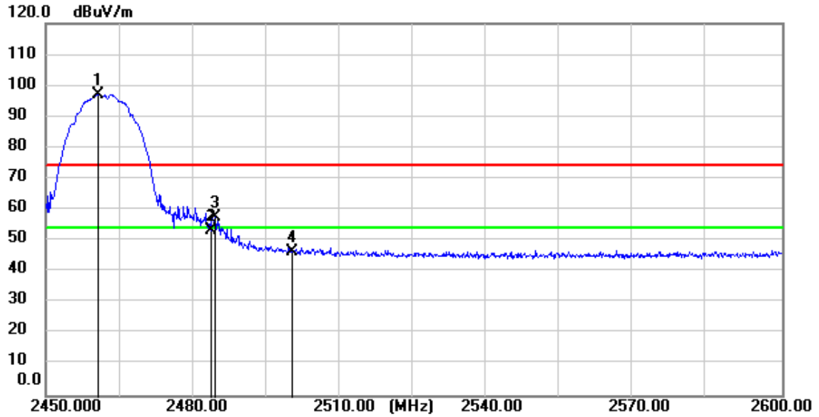
11b_TX_CH_11_Vertical_Peak
