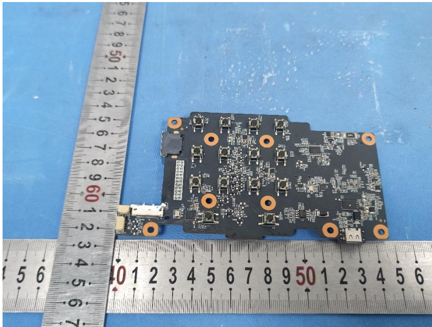
OET-131E-HMK-W
