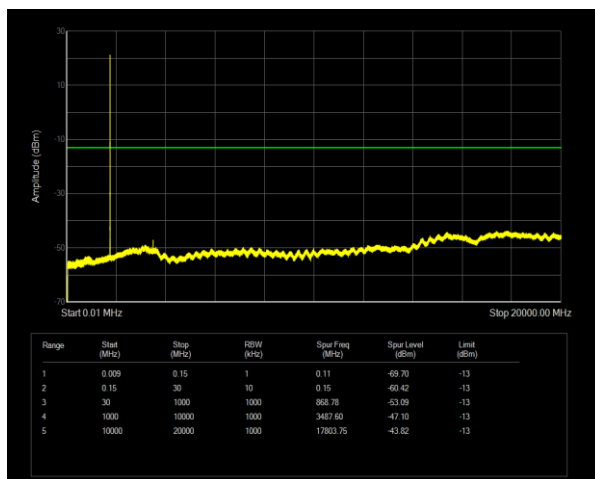
Band66 QPSK BW=3MHz Channel=132322 RB Size=1 Position=#0
