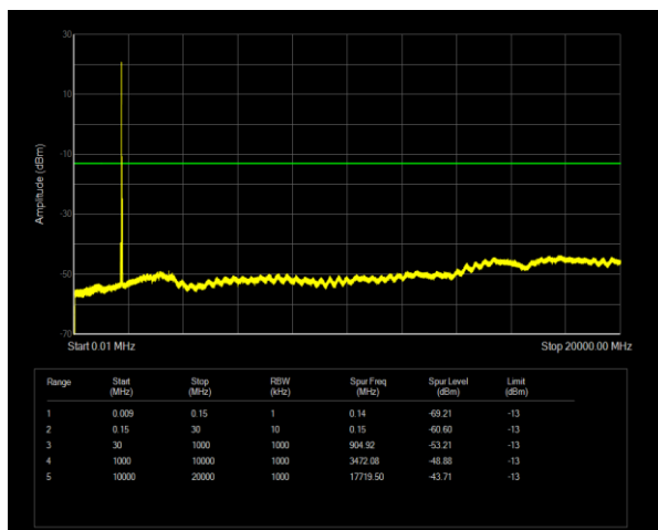
Band66 QPSK BW=20MHz Channel=132322 RB Size=1 Position=#0
