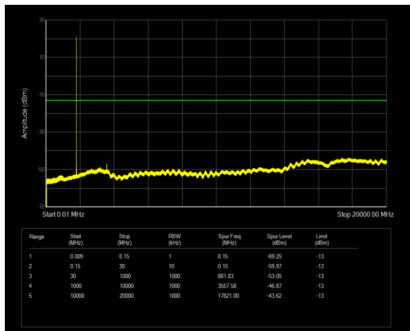
Band66 QPSK BW=1.4MHz Channel=132665 RB Size=1 Position=#0
