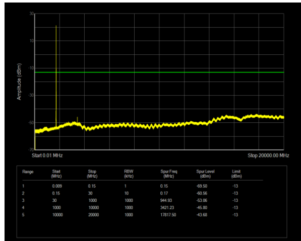
Band4 QPSK BW=5MHz Channel=19975 RB Size=1 Position=#0
