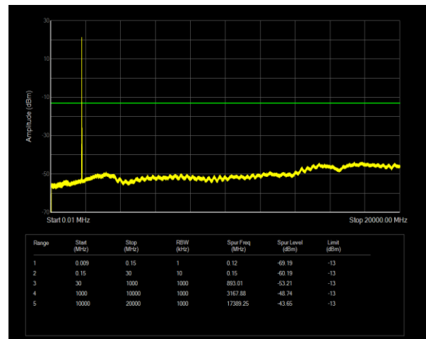
Band66 QPSK BW=10MHz Channel=132622 RB Size=1 Position=#0
