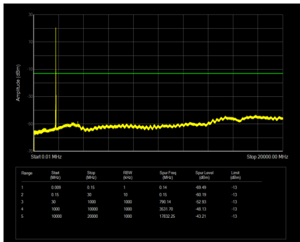
Band66 QPSK BW=15MHz Channel=132597 RB Size=1 Position=#0
