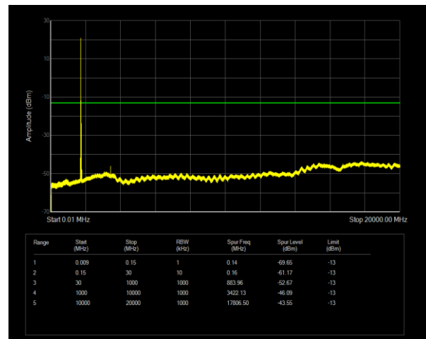
Band66 QPSK BW=20MHz Channel=132072 RB Size=1 Position=#0
