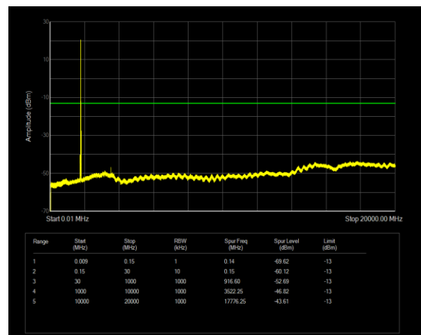
Band66 QPSK BW=20MHz Channel=132572 RB Size=1 Position=#0
