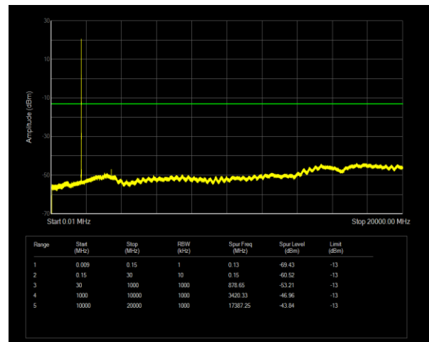
Band66 QPSK BW=3MHz Channel=131987 RB Size=1 Position=#0
