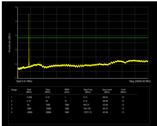
Band66 QPSK BW=15MHz Channel=132047 RB Size=1 Position=#0
