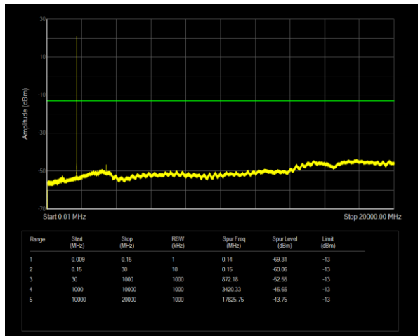
Band66 QPSK BW=1.4MHz Channel=131979 RB Size=1 Position=#0
