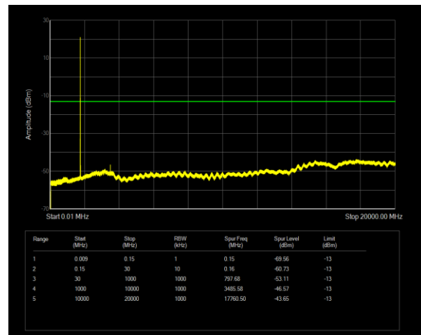
Band66 QPSK BW=5MHz Channel=132322 RB Size=1 Position=#0
