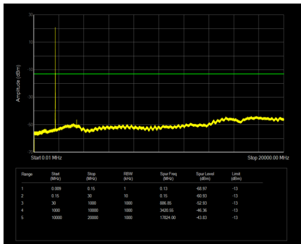
Band66 QPSK BW=5MHz Channel=131997 RB Size=1 Position=#0
