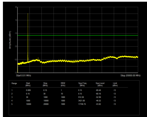
Band66 QPSK BW=10MHz Channel=132022 RB Size=1 Position=#0
