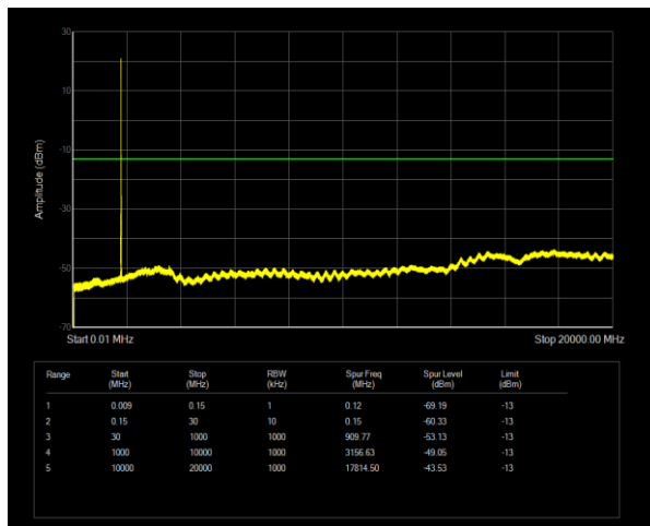
Band66 QPSK BW=5MHz Channel=132647 RB Size=1 Position=#0
