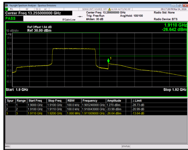
Band2 16QAM BW=10MHz HighChannel=19150 RB Size=27 Position=#Max
