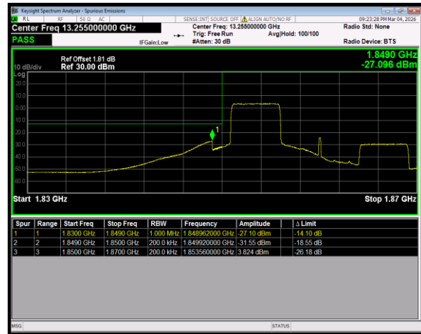
Band2 16QAM BW=20MHz LowChannel=18700 RB Size=27 Position=#0
