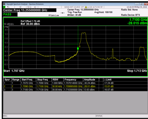
Band4 QPSK BW=3MHz LowChannel=19965 RB Size=1 Position=#0
