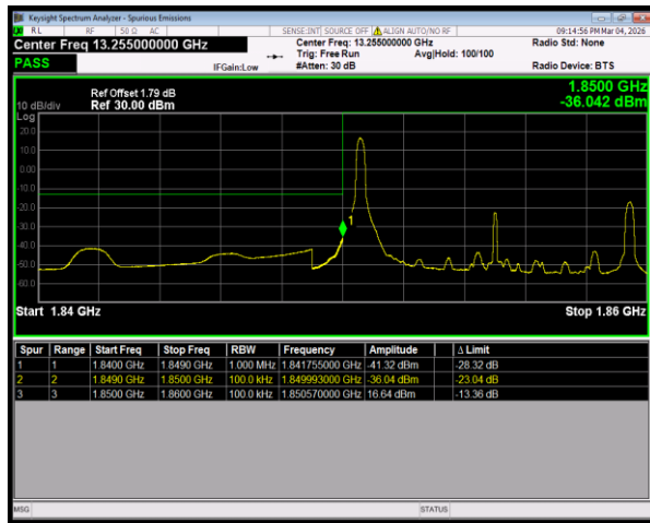
Band2 16QAM BW=10MHz LowChannel=18650 RB Size=1 Position=#0
