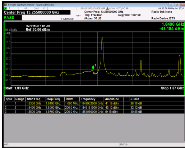
Band2 16QAM BW=20MHz LowChannel=18700 RB Size=1 Position=#0
