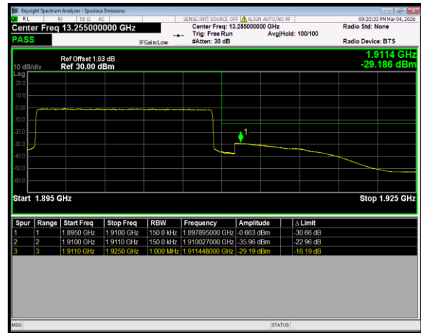
Band2 QPSK BW=15MHz HighChannel=19125 RB Size=75 Position=#0
