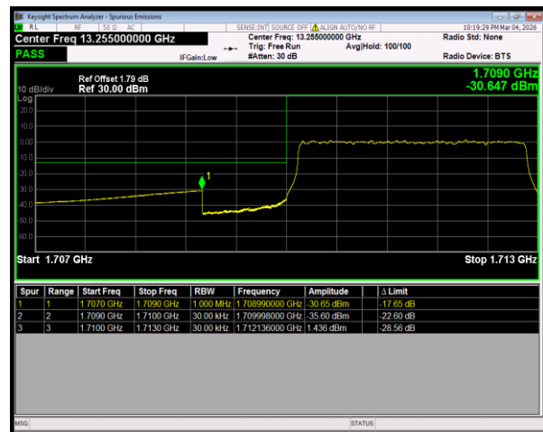
Band4 16QAM BW=3MHz LowChannel=19965 RB Size=15 Position=#0
