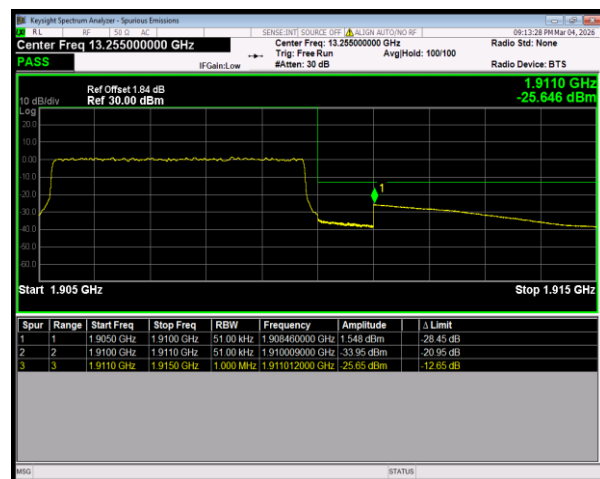
Band2 16QAM BW=5MHz HighChannel=19175 RB Size=25 Position=#0
