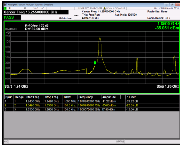
Band2 QPSK BW=10MHz LowChannel=18650 RB Size=1 Position=#0
