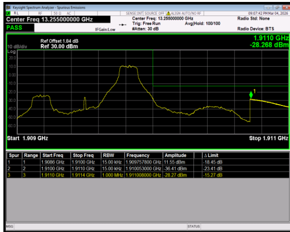
Band2 16QAM BW=1.4MHz HighChannel=19193 RB Size=1 Position=#Max
