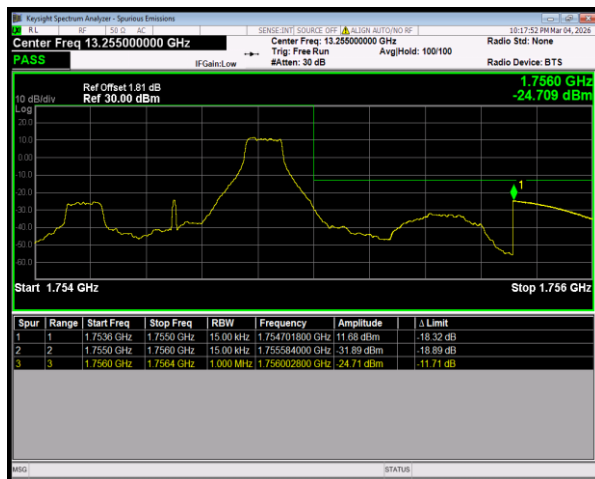
Band4 QPSK BW=1.4MHz HighChannel=20393 RB Size=1 Position=#Max
