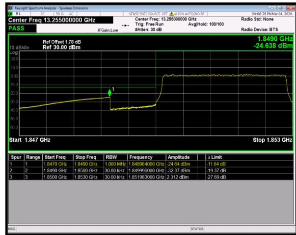
Band2 QPSK BW=3MHz LowChannel=18615 RB Size=15 Position=#0
