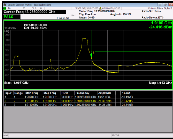
Band2 16QAM BW=3MHz HighChannel=19185 RB Size=1 Position=#Max
