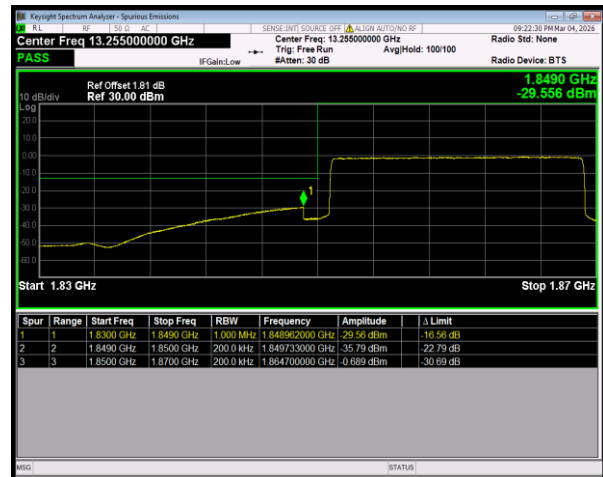
Band2 QPSK BW=20MHz LowChannel=18700 RB Size=100 Position=#0
