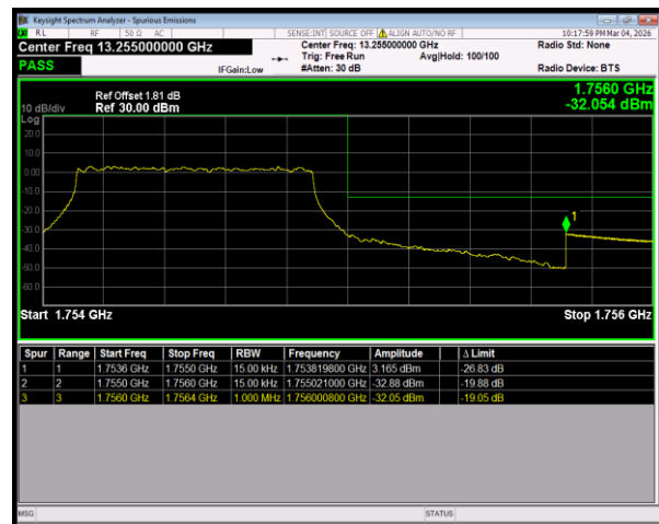
Band4 QPSK BW=1.4MHz HighChannel=20393 RB Size=6 Position=#0
