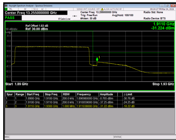
Band2 QPSK BW=20MHz HighChannel=19100 RB Size=100 Position=#0
