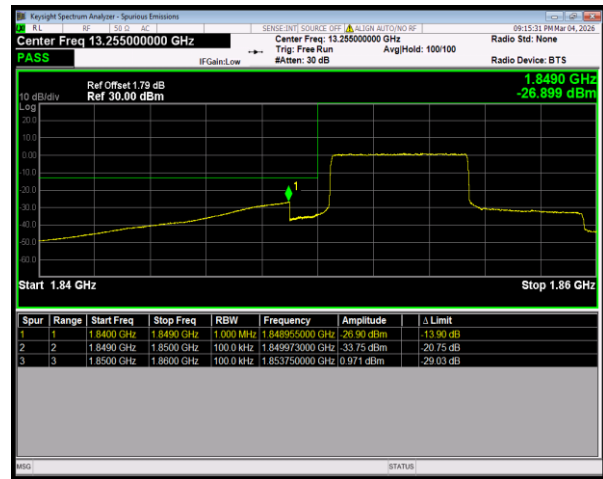
Band2 16QAM BW=10MHz LowChannel=18650 RB Size=27 Position=#0
