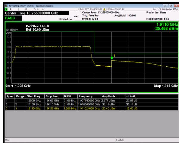
Band2 QPSK BW=5MHz HighChannel=19175 RB Size=25 Position=#0
