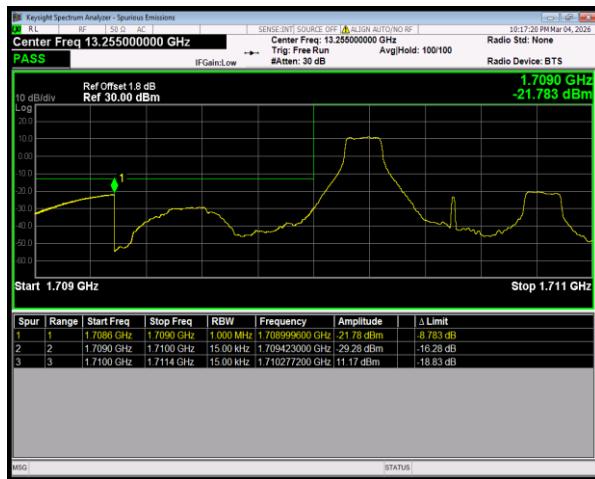
Band4 QPSK BW=1.4MHz LowChannel=19957 RB Size=1 Position=#0
