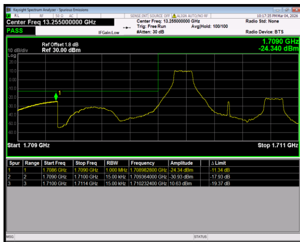
Band4 16QAM BW=1.4MHz LowChannel=19957 RB Size=1 Position=#0
