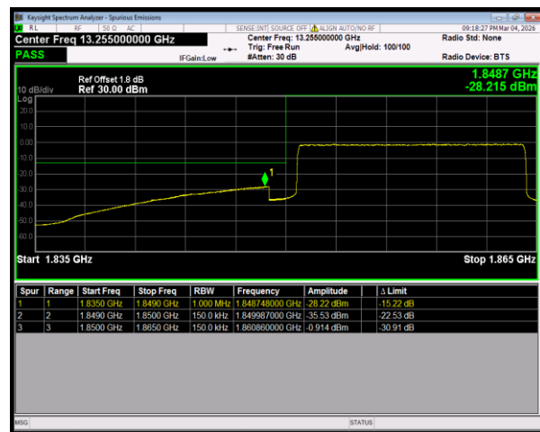
Band2 QPSK BW=15MHz LowChannel=18675 RB Size=75 Position=#0
