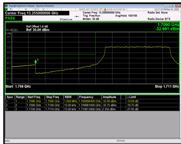
Band4 16QAM BW=1.4MHz LowChannel=19957 RB Size=6 Position=#0
