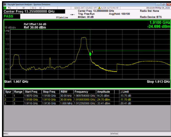
Band2 QPSK BW=3MHz HighChannel=19185 RB Size=1 Position=#Max
