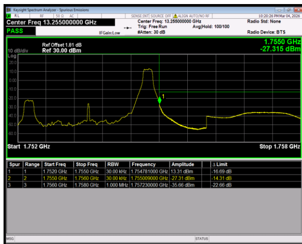
Band4 16QAM BW=3MHz HighChannel=20385 RB Size=1 Position=#Max
