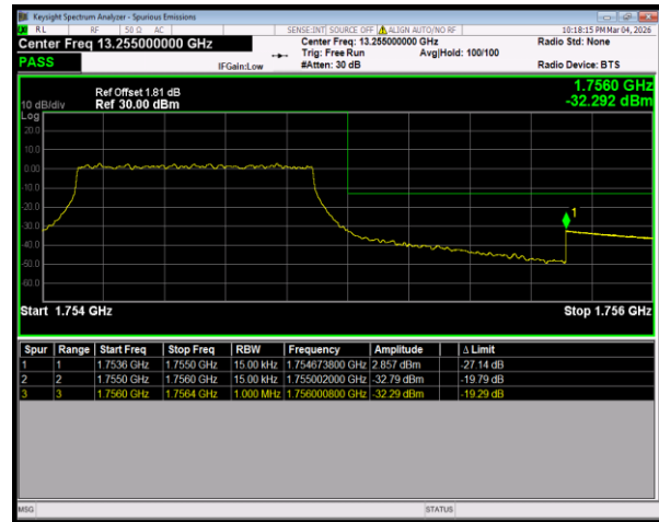
Band4 16QAM BW=1.4MHz HighChannel=20393 RB Size=6 Position=#0
