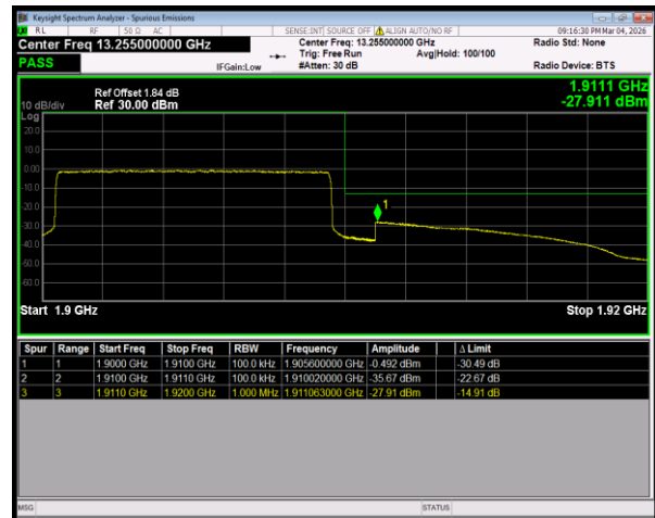
Band2 QPSK BW=10MHz HighChannel=19150 RB Size=50 Position=#0
