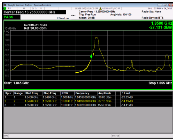
Band2 16QAM BW=5MHz LowChannel=18625 RB Size=1 Position=#0
