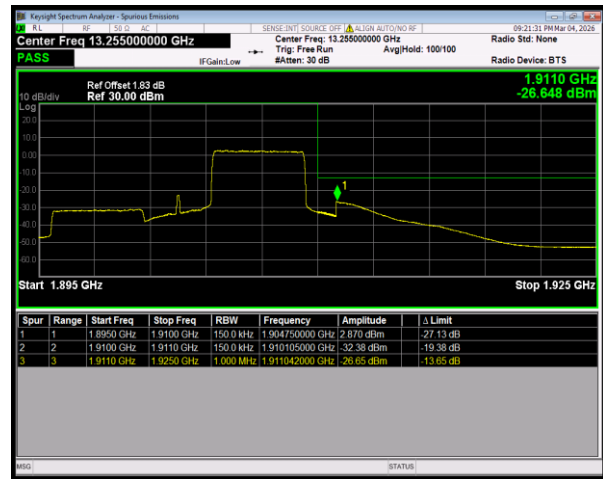
Band2 16QAM BW=15MHz HighChannel=19125 RB Size=27 Position=#Max
