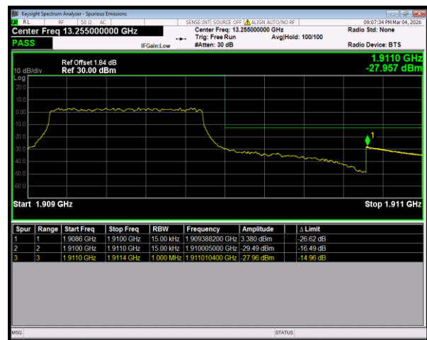
Band2 QPSK BW=1.4MHz HighChannel=19193 RB Size=6 Position=#0
