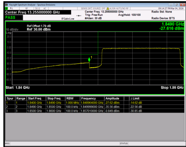
Band2 QPSK BW=10MHz LowChannel=18650 RB Size=50 Position=#0
