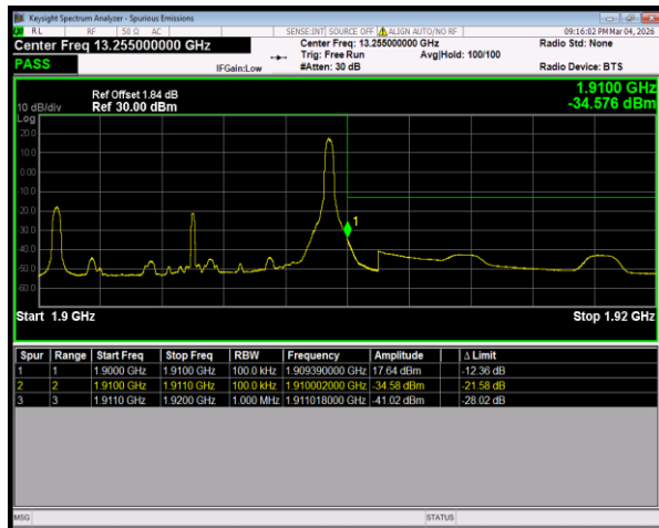
Band2 QPSK BW=10MHz HighChannel=19150 RB Size=1 Position=#Max
