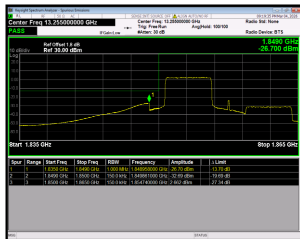
Band2 16QAM BW=15MHz LowChannel=18675 RB Size=27 Position=#0
