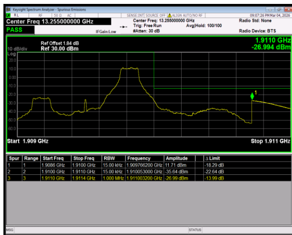
Band2 QPSK BW=1.4MHz HighChannel=19193 RB Size=1 Position=#Max
