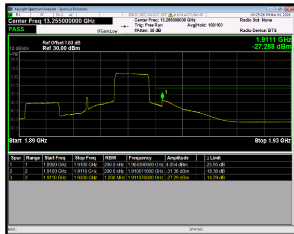
Band2 16QAM BW=20MHz HighChannel=19100 RB Size=27 Position=#Max
