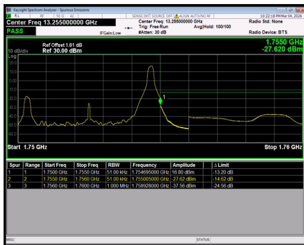
Band4 QPSK BW=5MHz HighChannel=20375 RB Size=1 Position=#Max
