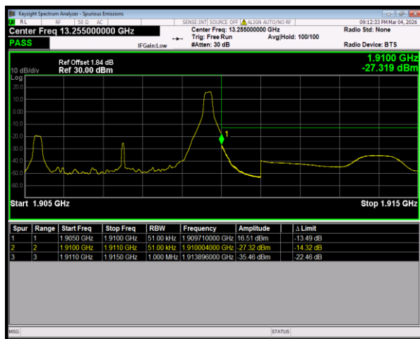
Band2 QPSK BW=5MHz HighChannel=19175 RB Size=1 Position=#Max
