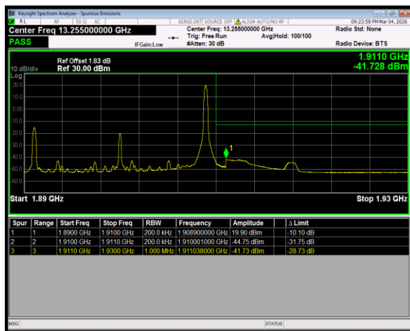
Band2 QPSK BW=20MHz HighChannel=19100 RB Size=1 Position=#Max
