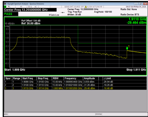
Band2 16QAM BW=1.4MHz HighChannel=19193 RB Size=6 Position=#0
