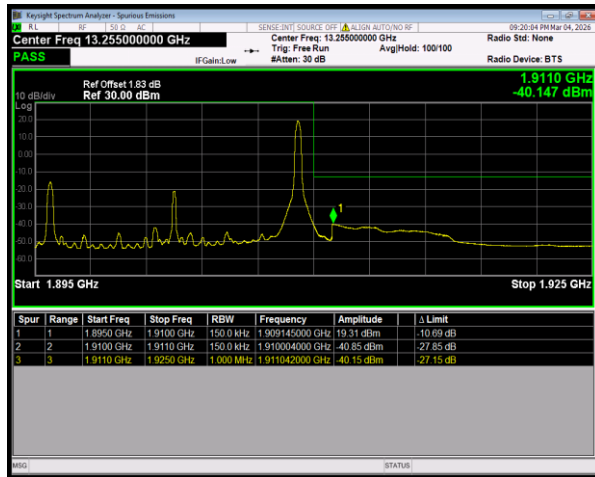
Band2 QPSK BW=15MHz HighChannel=19125 RB Size=1 Position=#Max
