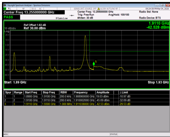
Band2 16QAM BW=20MHz HighChannel=19100 RB Size=1 Position=#Max
