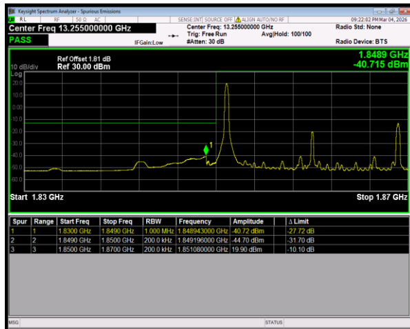
Band2 QPSK BW=20MHz LowChannel=18700 RB Size=1 Position=#0
