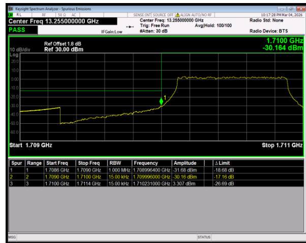
Band4 QPSK BW=1.4MHz LowChannel=19957 RB Size=6 Position=#0
