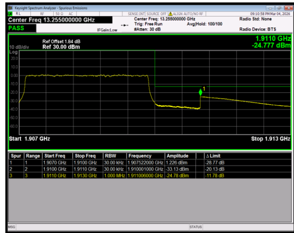
Band2 16QAM BW=3MHz HighChannel=19185 RB Size=15 Position=#0
