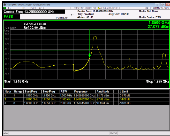
Band2 QPSK BW=5MHz LowChannel=18625 RB Size=1 Position=#0
