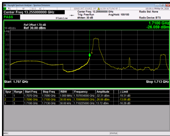
Band4 16QAM BW=3MHz LowChannel=19965 RB Size=1 Position=#0
