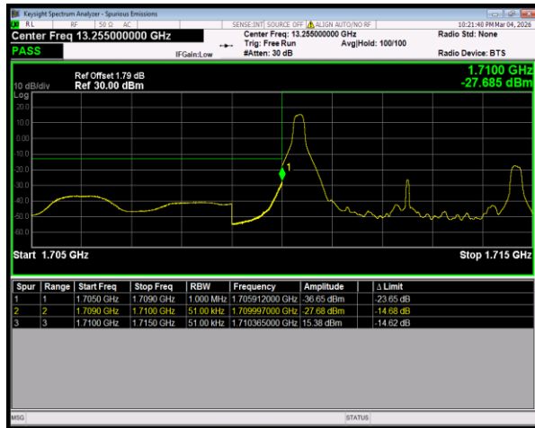
Band4 16QAM BW=5MHz LowChannel=19975 RB Size=1 Position=#0
