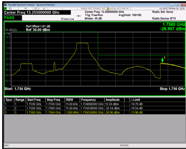
Band4 16QAM BW=1.4MHz HighChannel=20393 RB Size=1 Position=#Max
