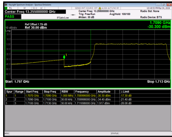
Band4 QPSK BW=3MHz LowChannel=19965 RB Size=15 Position=#0
