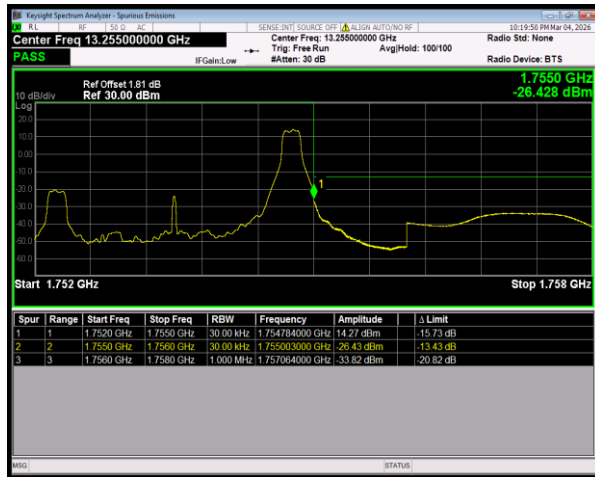
Band4 QPSK BW=3MHz HighChannel=20385 RB Size=1 Position=#Max
