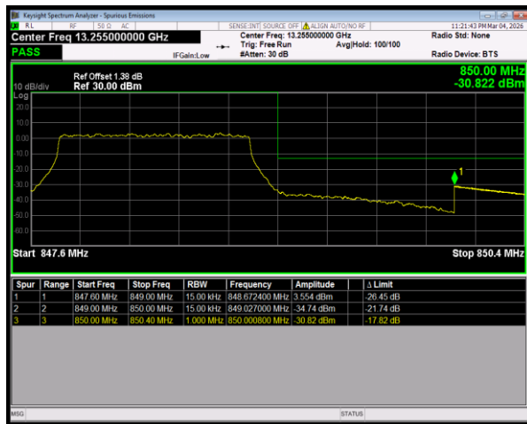
Band5 16QAM BW=1.4MHz HighChannel=20643 RB Size=6 Position=#0
