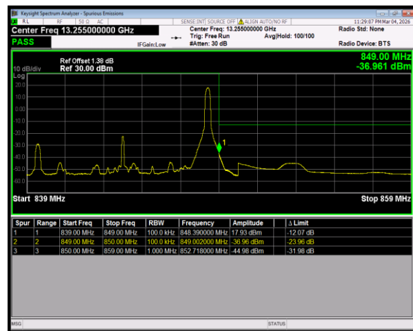
Band5 QPSK BW=10MHz HighChannel=20600 RB Size=1 Position=#Max
