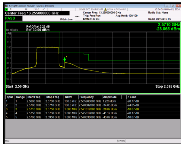
Band7 16QAM BW=5MHz HighChannel=21425 RB Size=25 Position=#0
