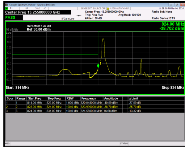
Band5 16QAM BW=10MHz LowChannel=20450 RB Size=1 Position=#0
