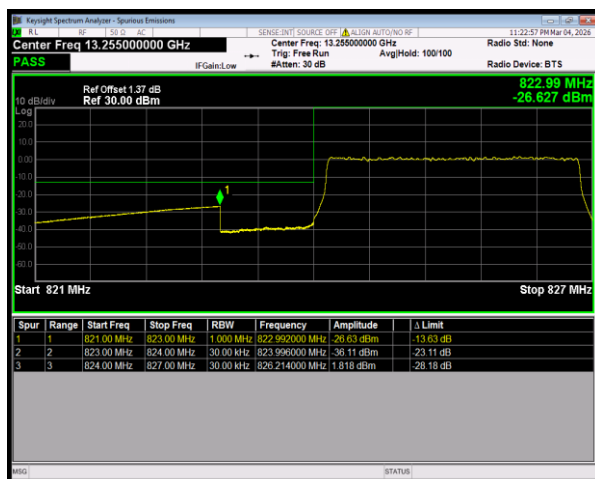
Band5 16QAM BW=3MHz LowChannel=20415 RB Size=15 Position=#0
