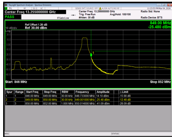
Band5 16QAM BW=3MHz HighChannel=20635 RB Size=1 Position=#Max
