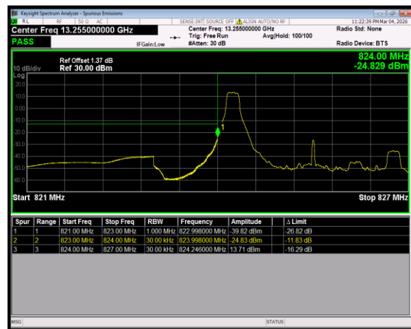
Band5 16QAM BW=3MHz LowChannel=20415 RB Size=1 Position=#0
