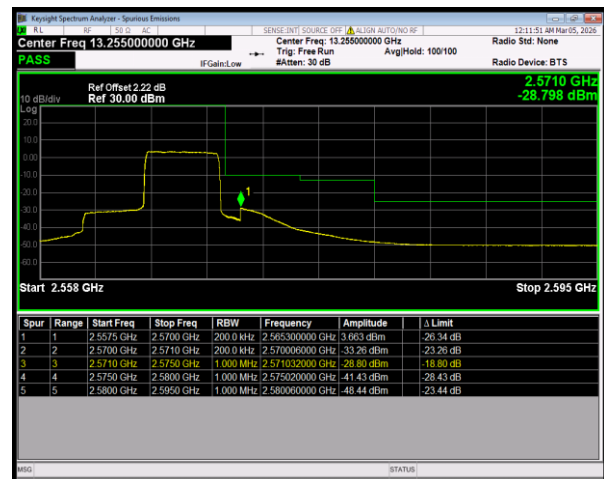
Band7 16QAM BW=10MHz HighChannel=21400 RB Size=27 Position=#Max
