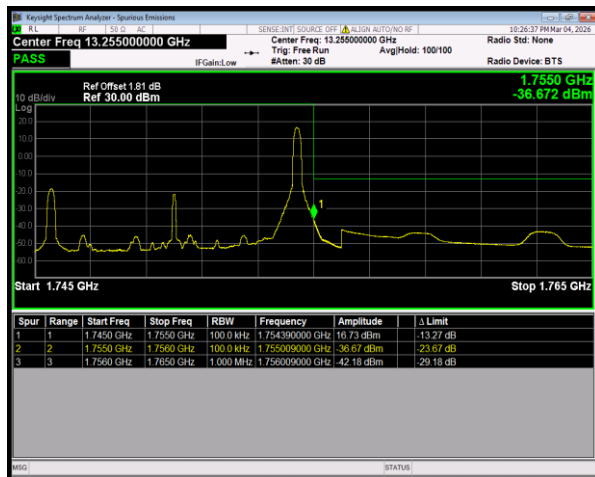
Band4 16QAM BW=10MHz HighChannel=20350 RB Size=1 Position=#Max
