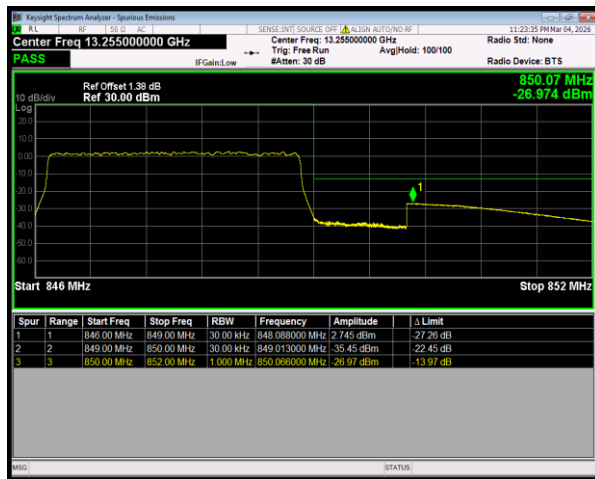
Band5 QPSK BW=3MHz HighChannel=20635 RB Size=15 Position=#0
