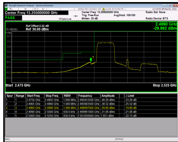
Band7 16QAM BW=20MHz LowChannel=20850 RB Size=27 Position=#0
