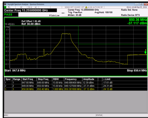
Band5 QPSK BW=1.4MHz HighChannel=20643 RB Size=1 Position=#Max
