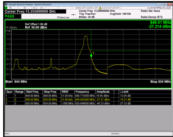
Band5 QPSK BW=5MHz HighChannel=20625 RB Size=1 Position=#Max
