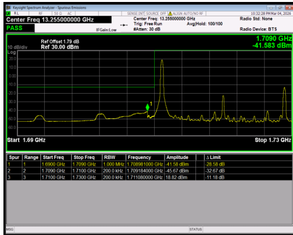
Band4 16QAM BW=20MHz LowChannel=20050 RB Size=1 Position=#0
