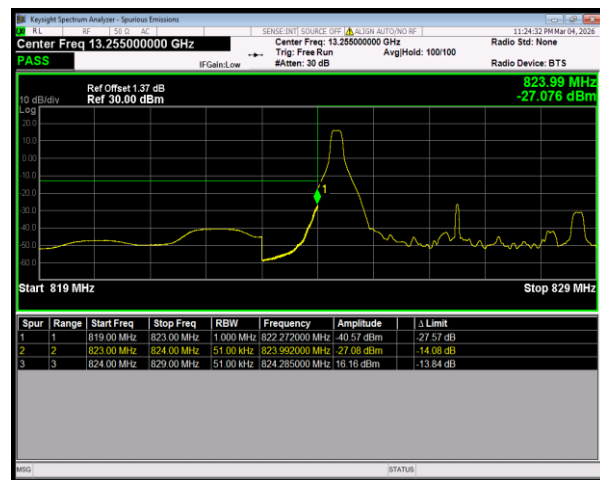
Band5 QPSK BW=5MHz LowChannel=20425 RB Size=1 Position=#0
