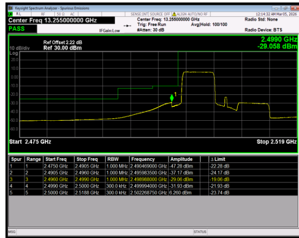
Band7 16QAM BW=15MHz LowChannel=20825 RB Size=27 Position=#0
