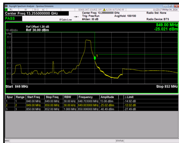
Band5 QPSK BW=3MHz HighChannel=20635 RB Size=1 Position=#Max
