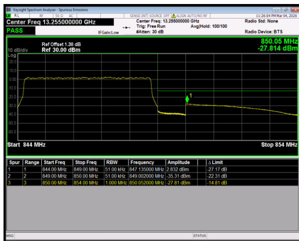
Band5 QPSK BW=5MHz HighChannel=20625 RB Size=25 Position=#0
