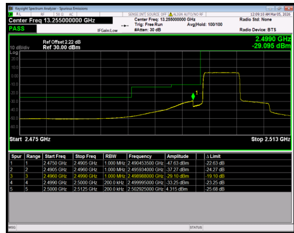
Band7 16QAM BW=10MHz LowChannel=20800 RB Size=27 Position=#0
