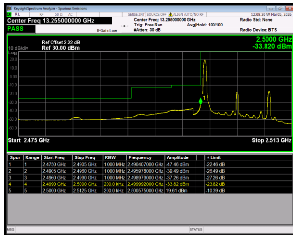
Band7 16QAM BW=10MHz LowChannel=20800 RB Size=1 Position=#0
