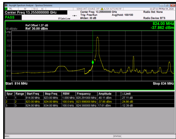
Band5 QPSK BW=10MHz LowChannel=20450 RB Size=1 Position=#0
