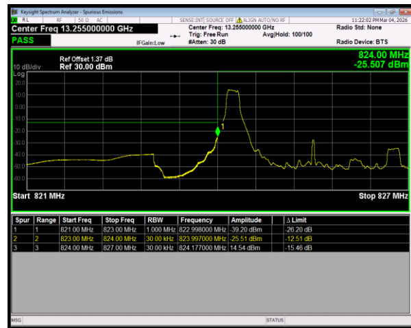
Band5 QPSK BW=3MHz LowChannel=20415 RB Size=1 Position=#0
