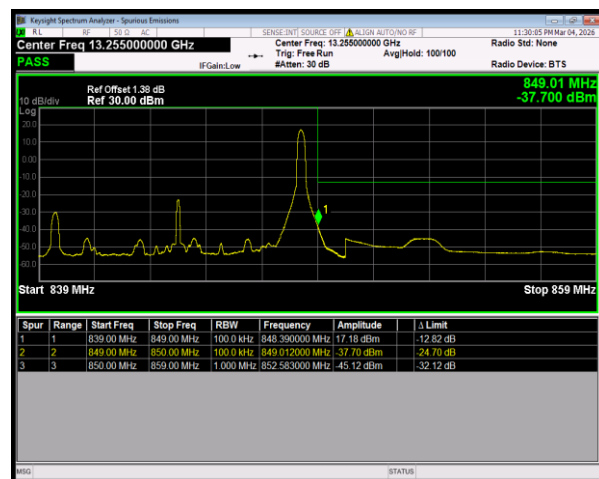
Band5 16QAM BW=10MHz HighChannel=20600 RB Size=1 Position=#Max
