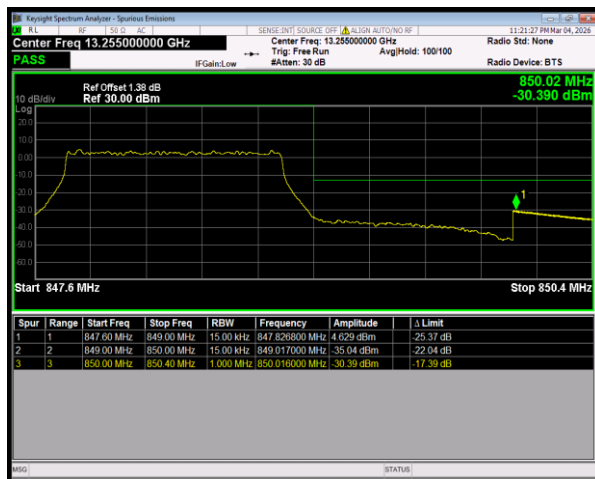
Band5 QPSK BW=1.4MHz HighChannel=20643 RB Size=6 Position=#0
