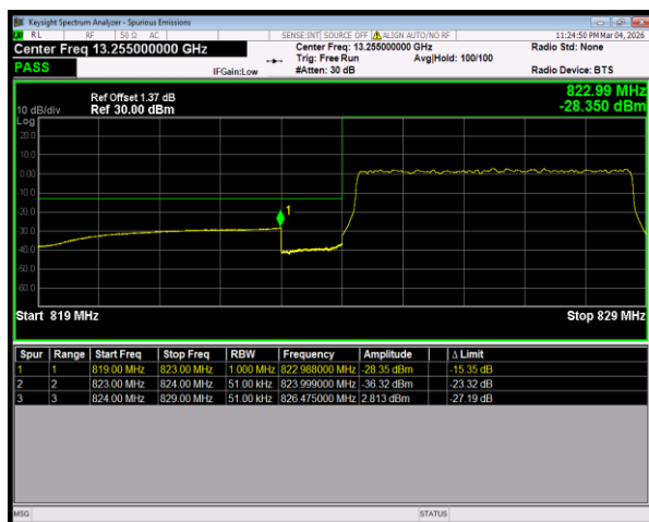
Band5 QPSK BW=5MHz LowChannel=20425 RB Size=25 Position=#0
