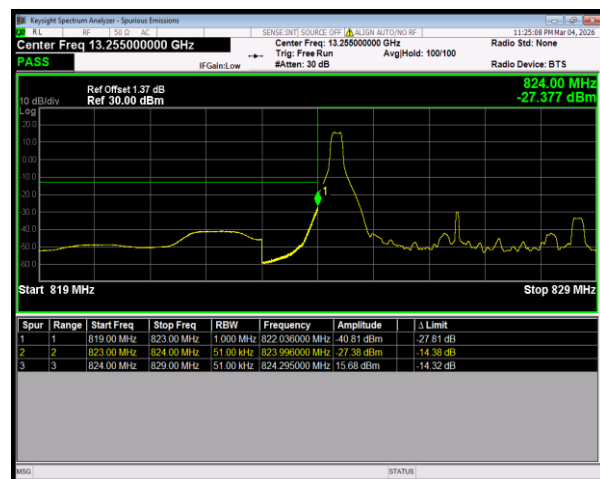
Band5 16QAM BW=5MHz LowChannel=20425 RB Size=1 Position=#0
