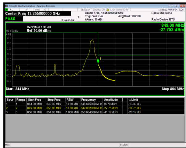
Band5 16QAM BW=5MHz HighChannel=20625 RB Size=1 Position=#Max
