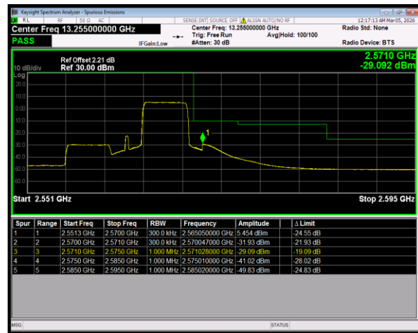
Band7 16QAM BW=15MHz HighChannel=21375 RB Size=27 Position=#Max
