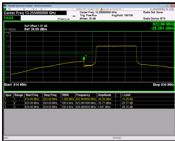
Band5 16QAM BW=10MHz LowChannel=20450 RB Size=27 Position=#0
