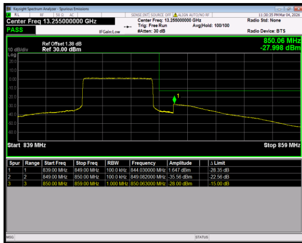
Band5 16QAM BW=10MHz HighChannel=20600 RB Size=27 Position=#Max
