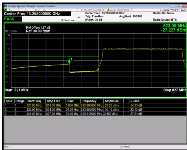
Band5 QPSK BW=3MHz LowChannel=20415 RB Size=15 Position=#0
