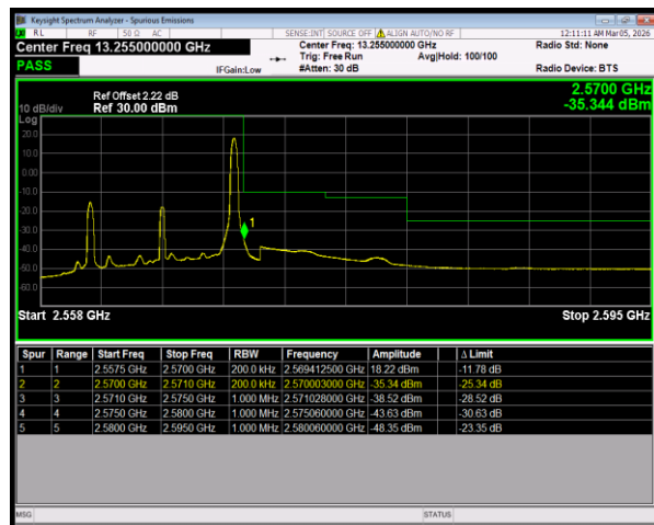
Band7 16QAM BW=10MHz HighChannel=21400 RB Size=1 Position=#Max
