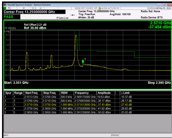
Band7 QPSK BW=15MHz HighChannel=21375 RB Size=1 Position=#Max
