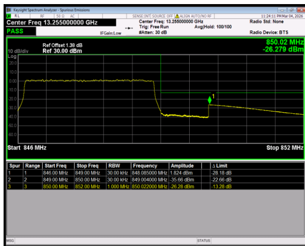
Band5 16QAM BW=3MHz HighChannel=20635 RB Size=15 Position=#0
