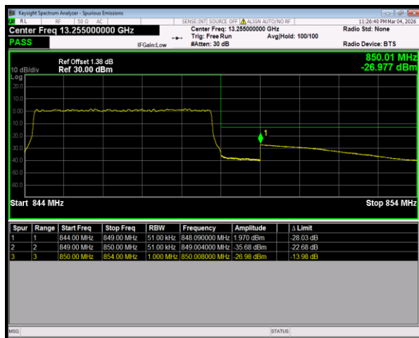
Band5 16QAM BW=5MHz HighChannel=20625 RB Size=25 Position=#0
