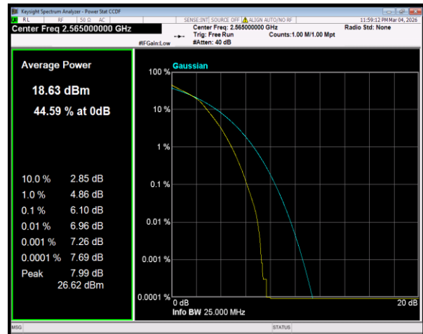
Band7 16QAM BW=10MHz Channel=21400 RB Size=27 Position=#0
