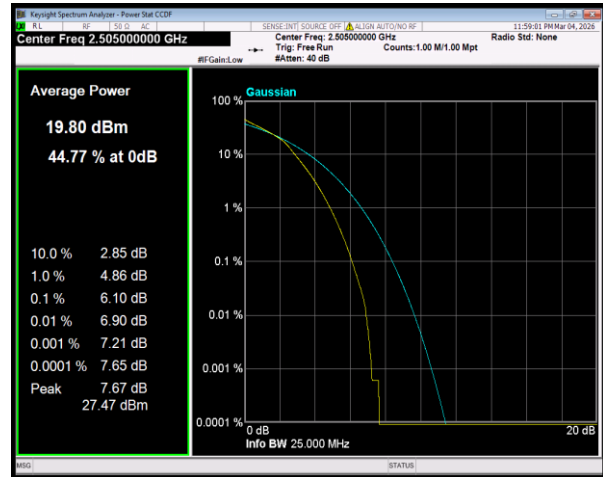
Band7 16QAM BW=10MHz Channel=20800 RB Size=27 Position=#0
