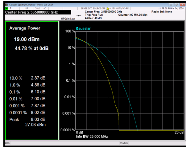
Band7 16QAM BW=10MHz Channel=21100 RB Size=27 Position=#0
