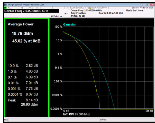
Band7 16QAM BW=20MHz Channel=21100 RB Size=27 Position=#0
