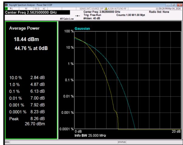
Band7 16QAM BW=15MHz Channel=21375 RB Size=27 Position=#0
