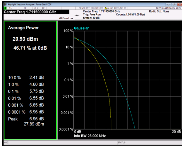
Band66 QPSK BW=3MHz Channel=131987 RB Size=15 Position=#0
