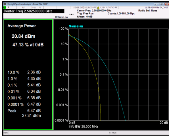
Band7 QPSK BW=5MHz Channel=20775 RB Size=25 Position=#0
