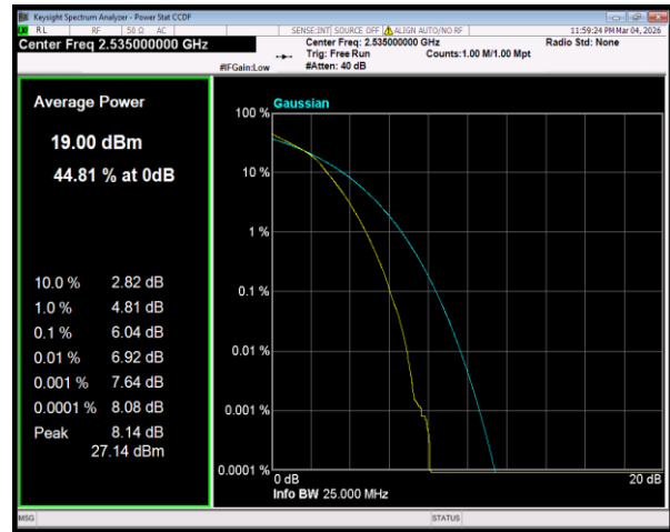
Band7 16QAM BW=15MHz Channel=21100 RB Size=27 Position=#0
