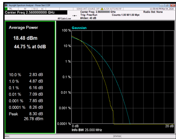
Band7 16QAM BW=20MHz Channel=21350 RB Size=27 Position=#0
