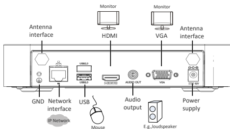
Figure 4-1 NVR Interfaces
