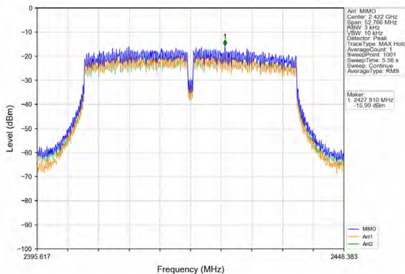
802.11n(HT40)_LCH_2422MHz_MIMO NTN
