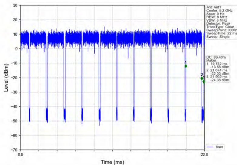
802.11n(HT20)_MCH_5200MHz_Ant1_NTNV
