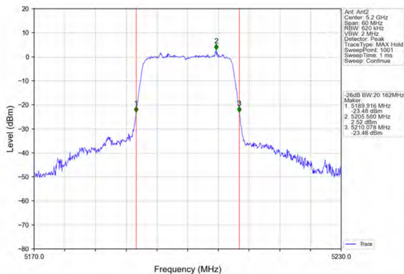
802.11ac(VHT20)_MCH_5200MHz_Ant2_NTNV
