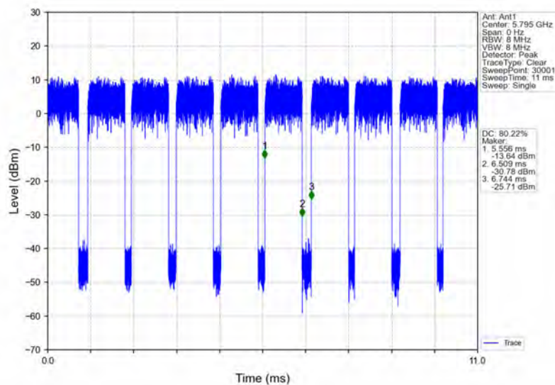
802.11ac(VHT40)_HCH_5795MHz_Ant1_NTNV
