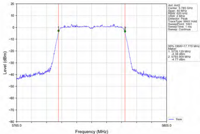
802.11ac(VHT20)_MCH_5785MHz_Ant2_NTNV
