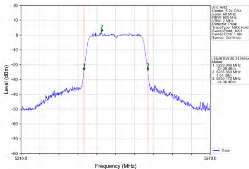
802.11n(HT20)_HCH_5240MHz_Ant2_NTNV
