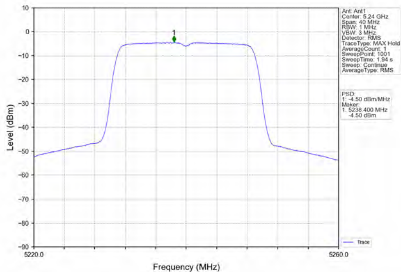
802.11ac(VHT20)_HCH_5240MHz_Ant1_NTNV
