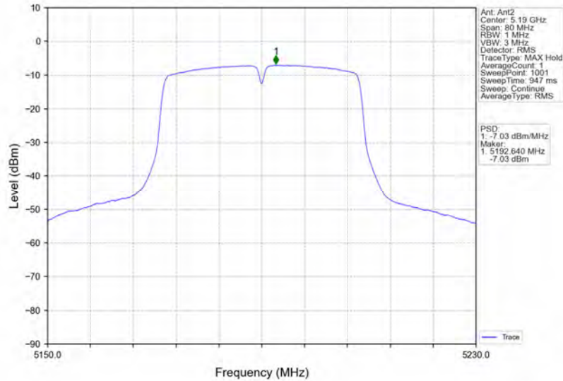
802.11n(HT40)_LCH_5190MHz_MIMO_NTNV
