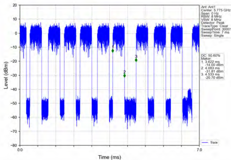
802.11ac(VHT80)_MCH_5775MHz_Ant1_NTNV
