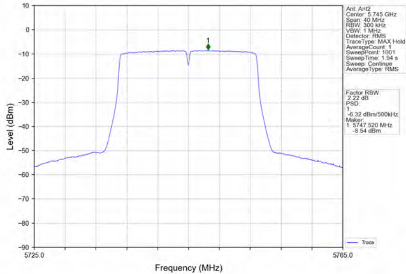
802.11ac(VHT20)_LCH_5745MHz_MIMO_NTNV
