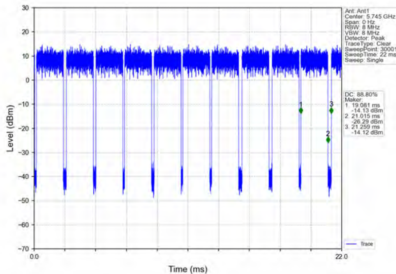
802.11ac(VHT20)_LCH_5745MHz_Ant1_NTNV
