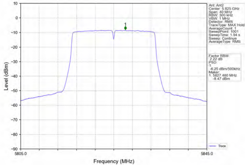
802.11ac(VHT20)_HCH_5825MHz_MIMO_NTNV
