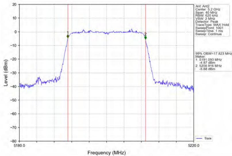
802.11ac(VHT20)_MCH_5200MHz_Ant2_NTNV
