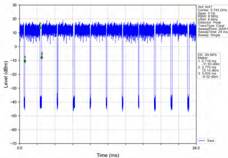
802.11a_LCH_5745MHz_Ant1_NTNV
