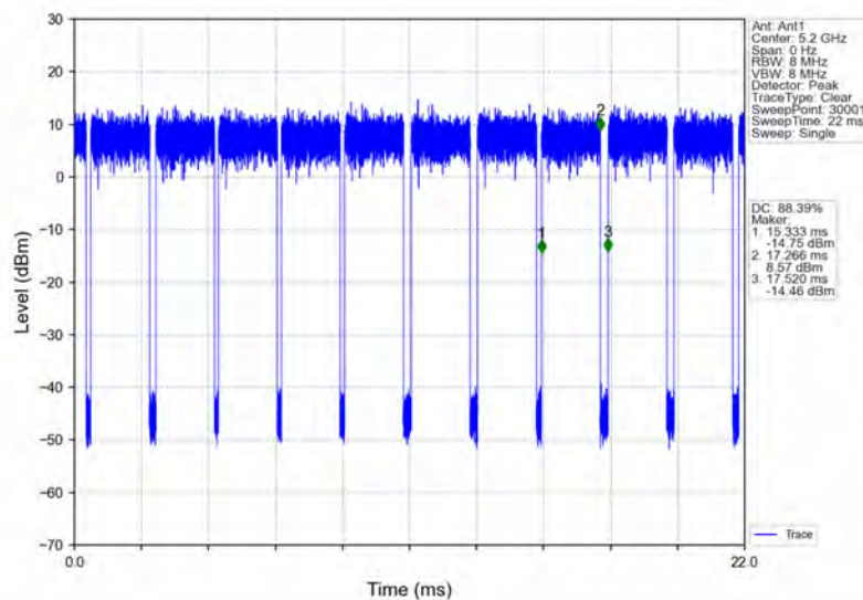
802.11ac(VHT20)_MCH_5200MHz_Ant1_NTNV
