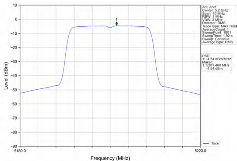
802.11n(HT20)_MCH_5200MHz_Ant1_NTNV
