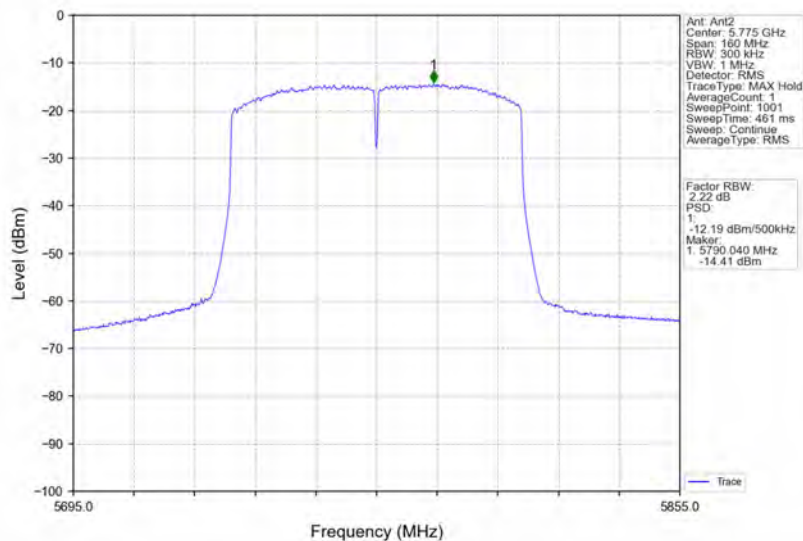
802.11ac(VHT80)_MCH_5775MHz_Ant2_NTNV
