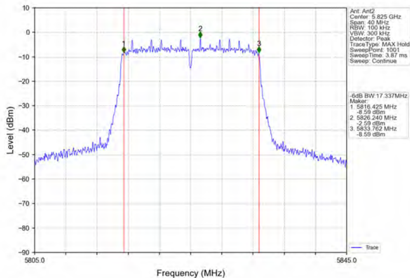
802.11ac(VHT20)_HCH_5825MHz_Ant2_NTNV
