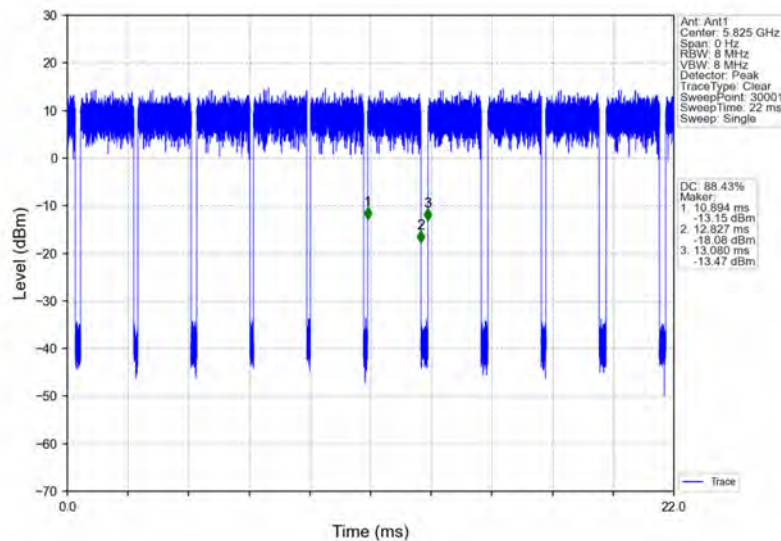
802.11ac(VHT20)_HCH_5825MHz_Ant1_NTNV
