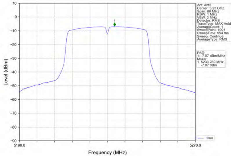
802.11ac(VHT40)_HCH_5230MHz_MIMO_NTNV
