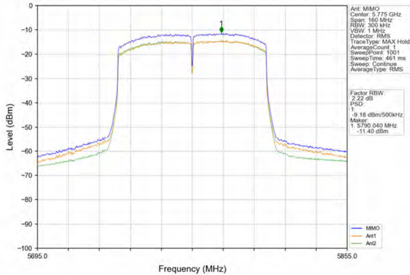
802.11ac(VHT80)_MCH_5775MHz_MIMO_NTNV
