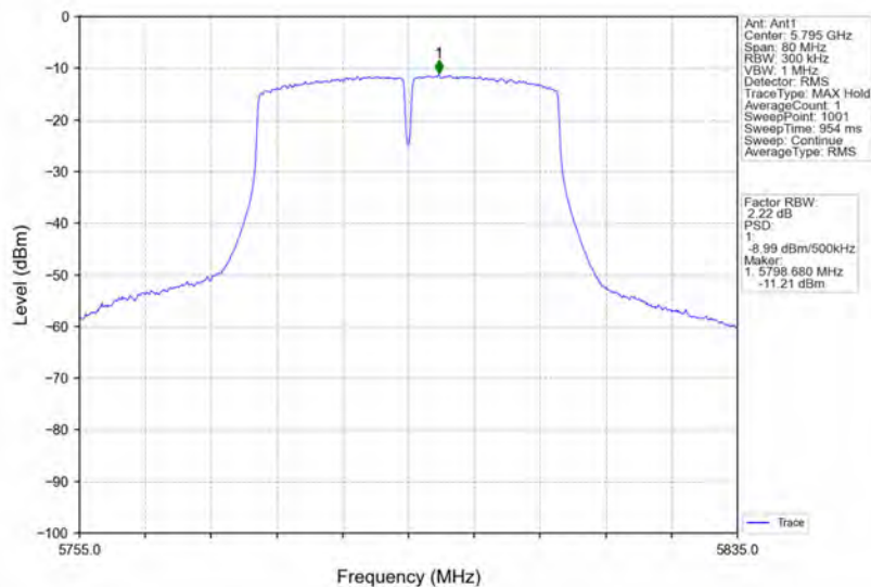
802.11ac(VHT40)_HCH_5795MHz_Ant1_NTNV
