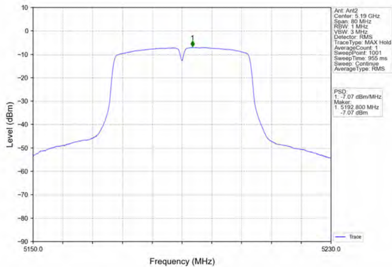
802.11ac(VHT40)_LCH_5190MHz_Ant2_NTNV
