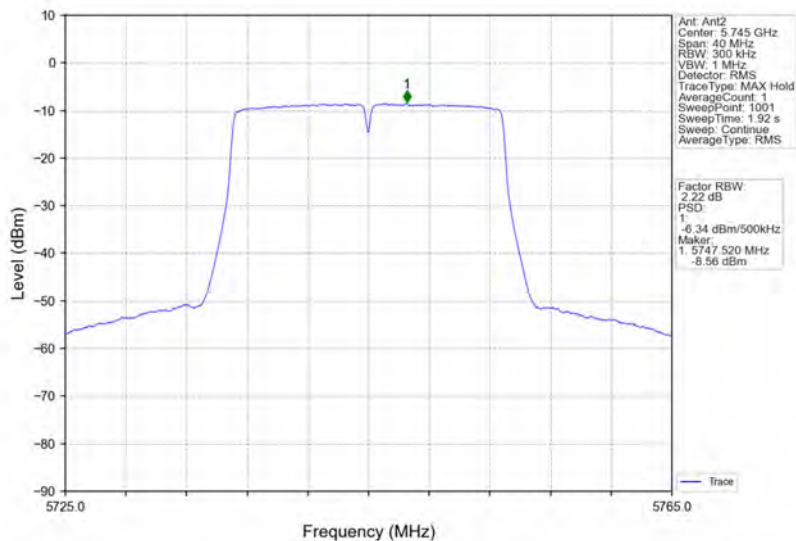
802.11n(HT20)_LCH_5745MHz_Ant2_NTNV
