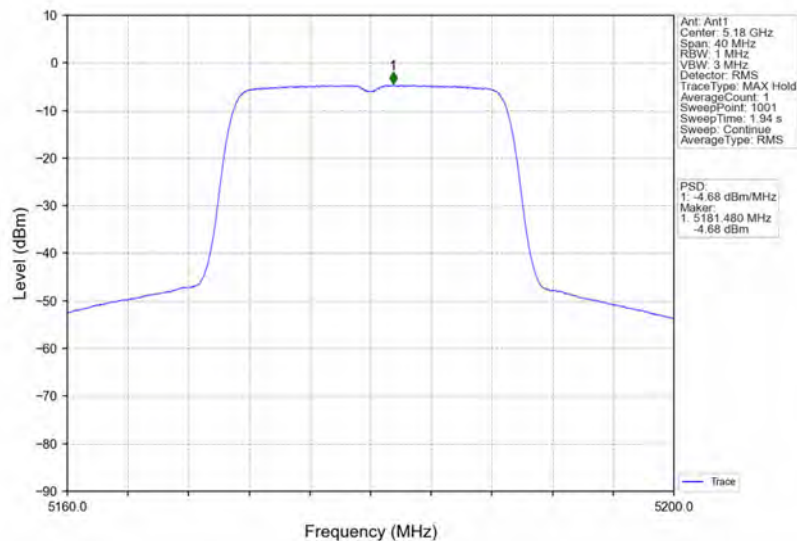
802.11ac(VHT20)_LCH_5180MHz_Ant1_NTNV
