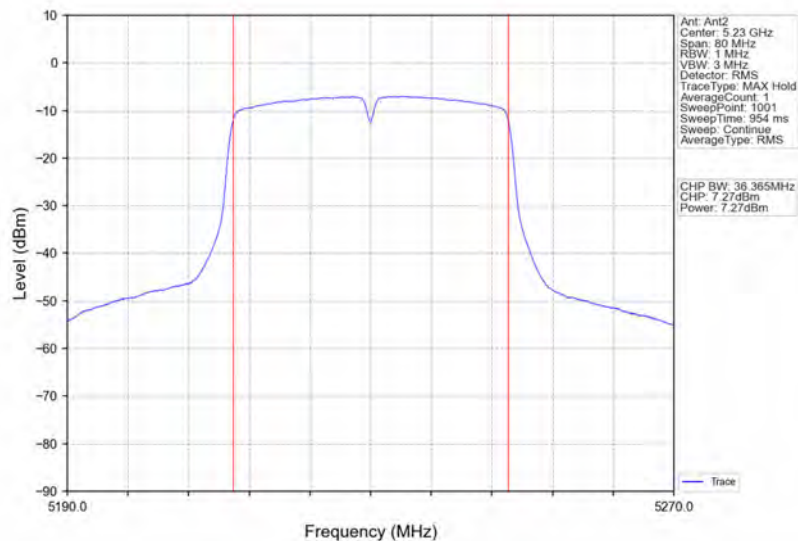
802.11ac(VHT40)_HCH_5230MHz_Ant2_NTNV
