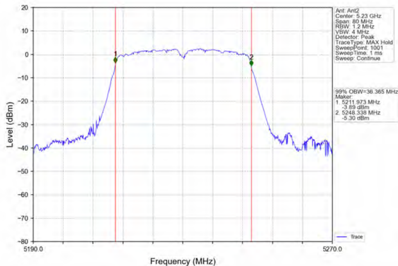
802.11ac(VHT40)_HCH_5230MHz_Ant2_NTNV
