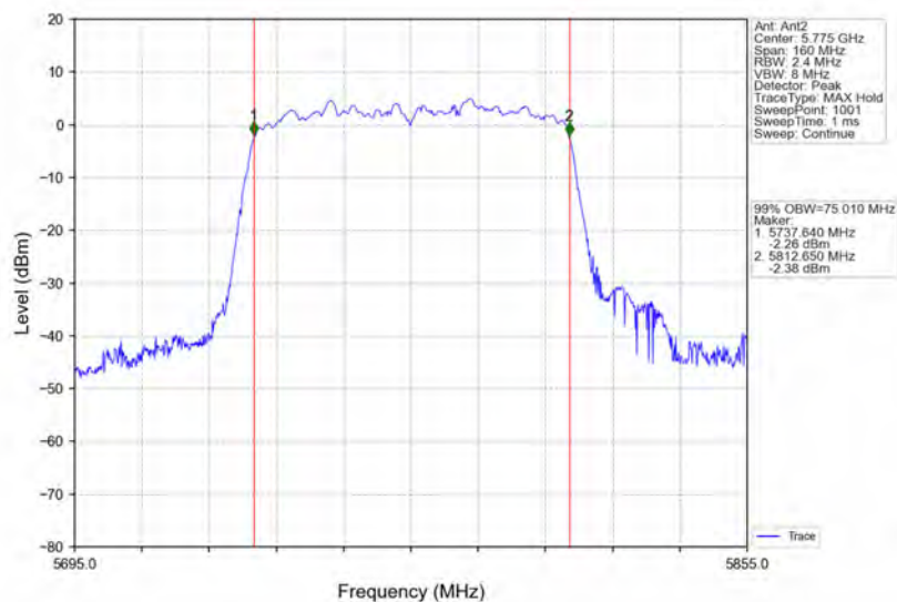
802.11ac(VHT80)_MCH_5775MHz_Ant2_NTNV
