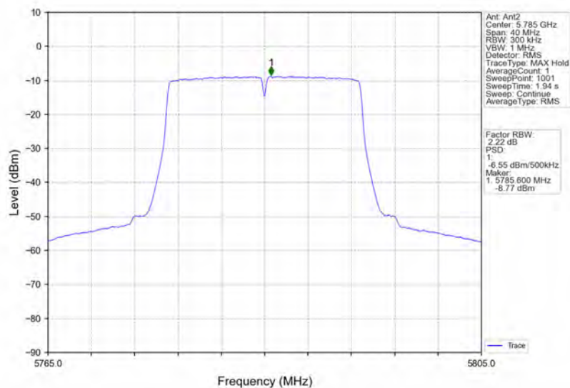
802.11ac(VHT20)_MCH_5785MHz_Ant2_NTNV
