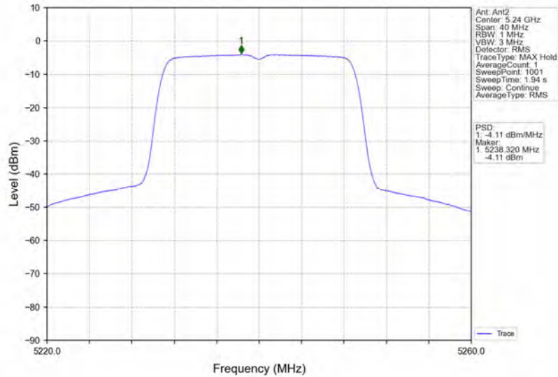
802.11ac(VHT20)_HCH_5240MHz_MIMO_NTNV
