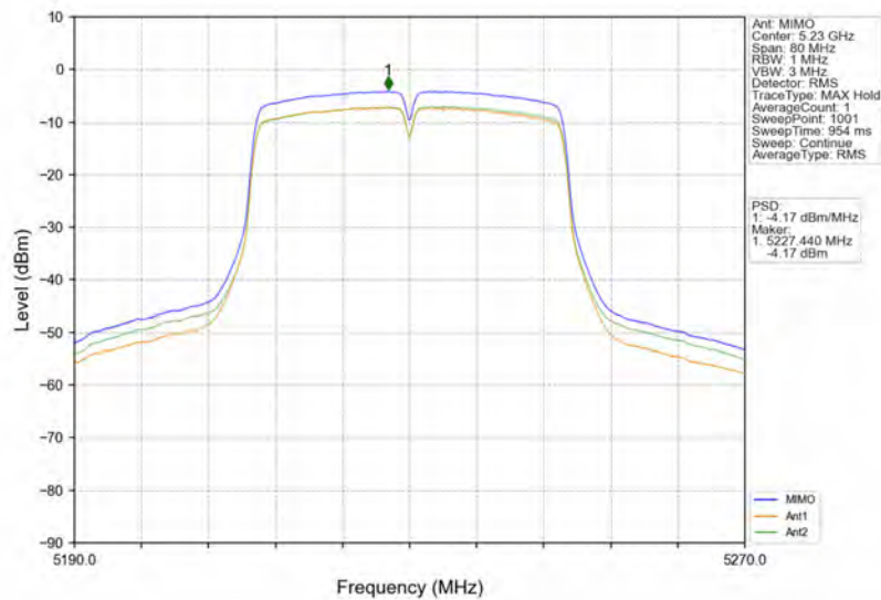
802.11ac(VHT40)_HCH_5230MHz_MIMO_NTNV
