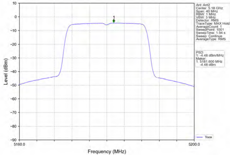
802.11ac(VHT20)_LCH_5180MHz_MIMO_NTNV
