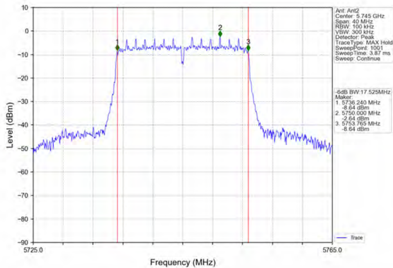
802.11ac(VHT20)_LCH_5745MHz_Ant2_NTNV
