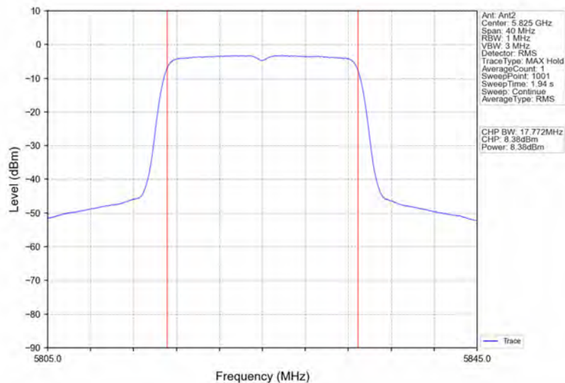
802.11ac(VHT20)_HCH_5825MHz_Ant2_NTNV
