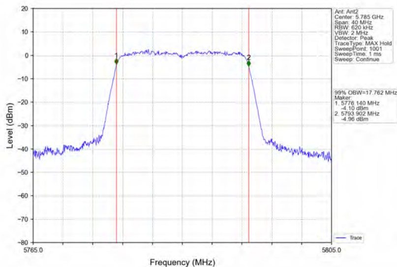
802.11n(HT20)_MCH_5785MHz_Ant2_NTNV
