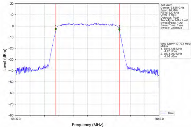
802.11ac(VHT20)_HCH_5825MHz_Ant2_NTNV
