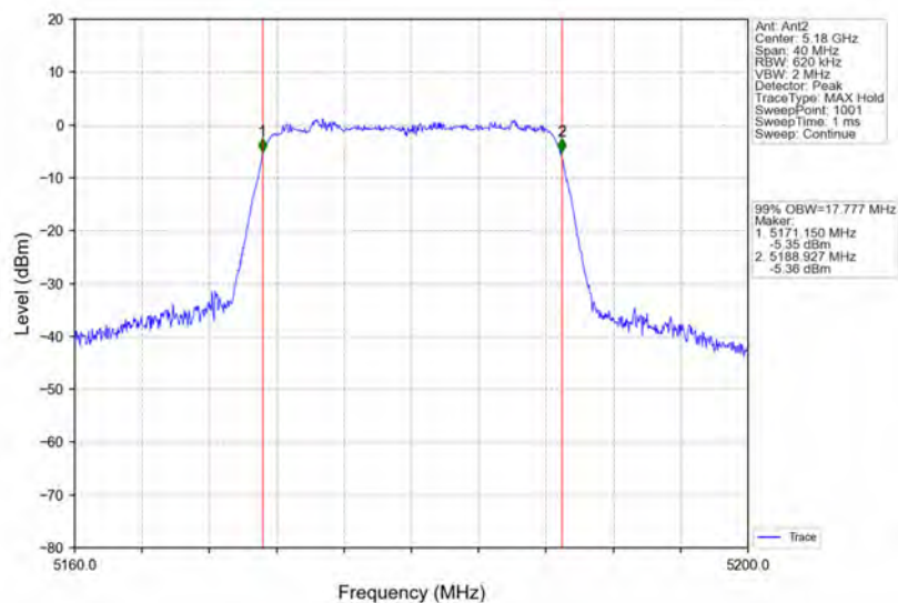
802.11ac(VHT20)_LCH_5180MHz_Ant2_NTNV
