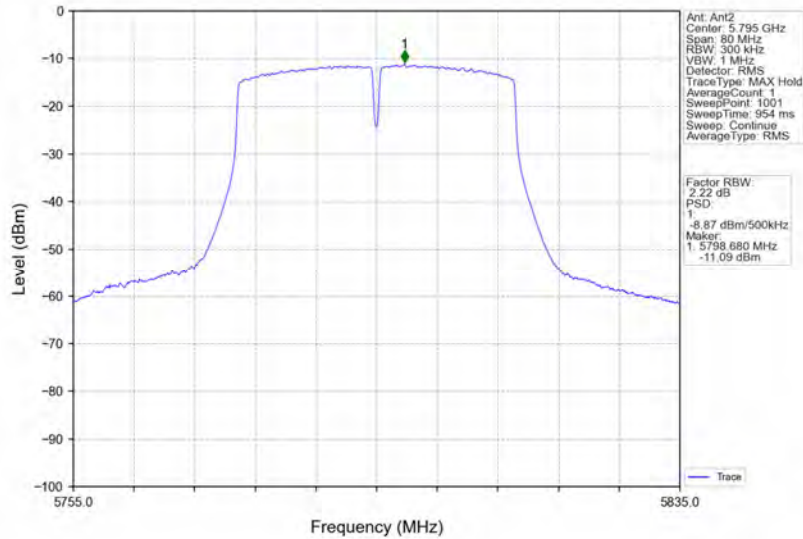
802.11ac(VHT40)_HCH_5795MHz_MIMO_NTNV
