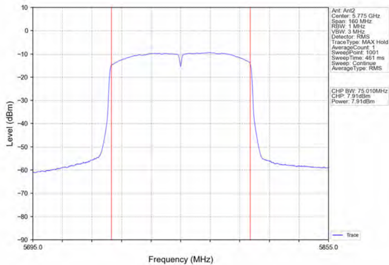
802.11ac(VHT80)_MCH_5775MHz_Ant2_NTNV
