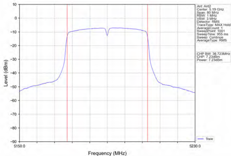
802.11ac(VHT40)_LCH_5190MHz_Ant2_NTNV
