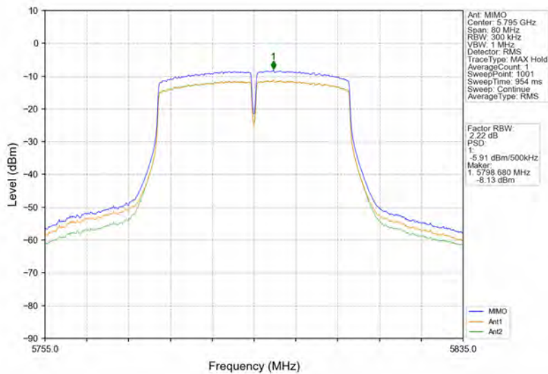
802.11ac(VHT40)_HCH_5795MHz_MIMO_NTNV
