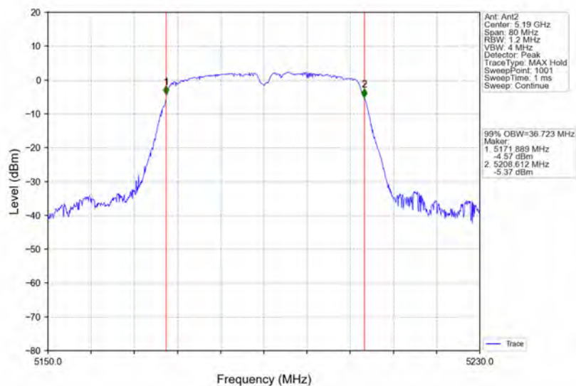
802.11ac(VHT40)_LCH_5190MHz_Ant2_NTNV
