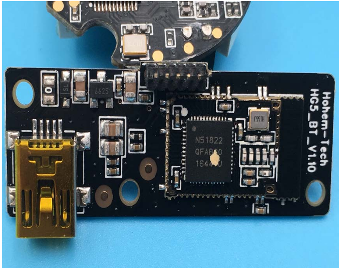
2. Mainboard front view
