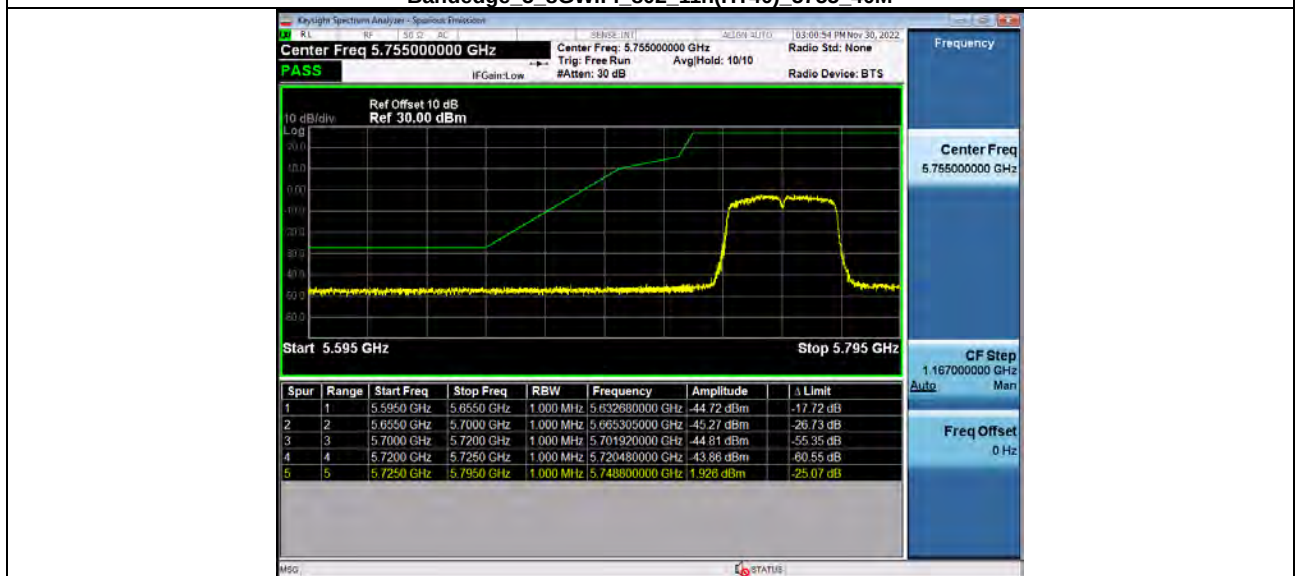
Bandedge 5 8GWiFi 802_11n(HT40) 5755 40M
