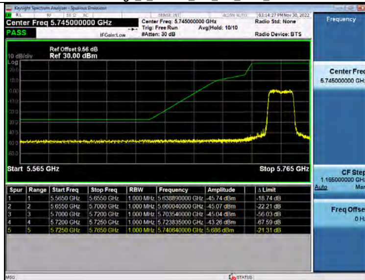
Bandedge 5 8GWiFi 802_11a 5745 20M
