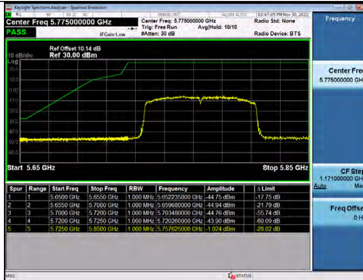
Bandedge 5 8GWiFi 802_11ac(VHT80) 5775 80M up
