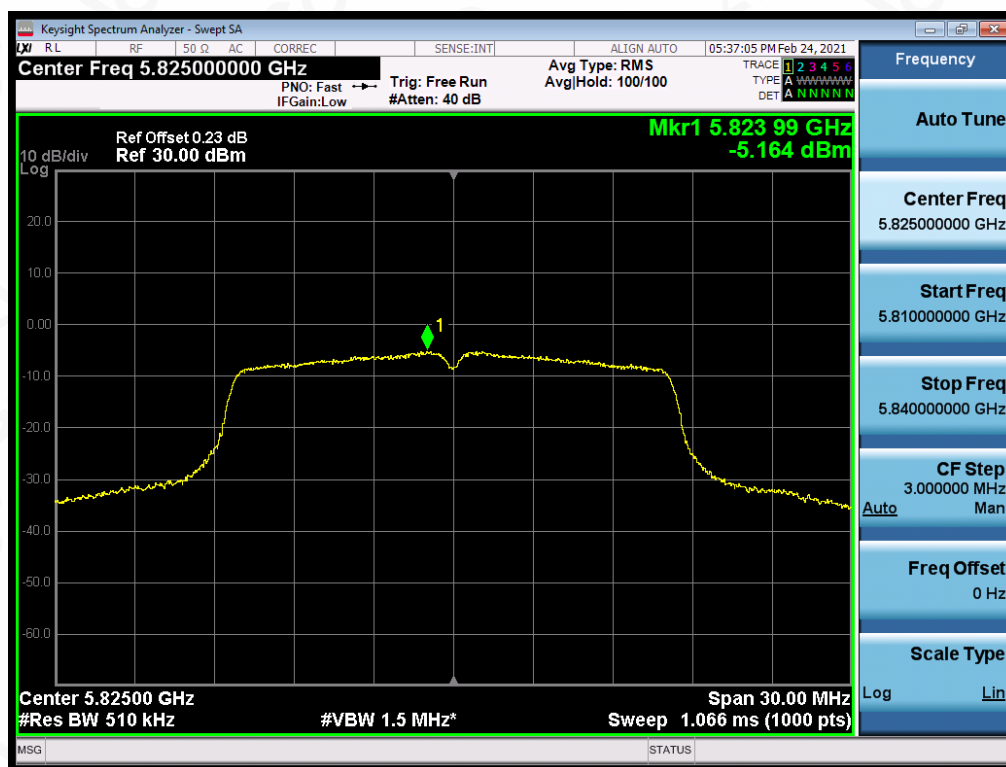
Test_Graph_802.11a_ANT1_5825_6Mbps_PSD
