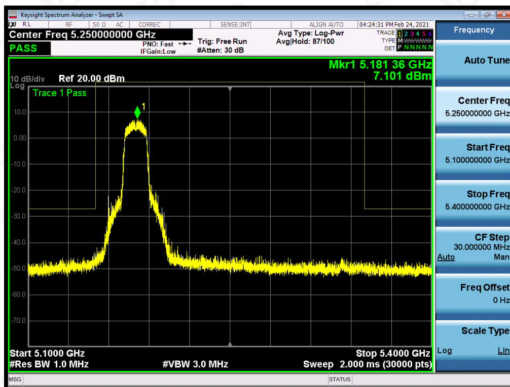
Test_Graph_802.11a_ANT1_5180_6Mbps_Frequency Band3
