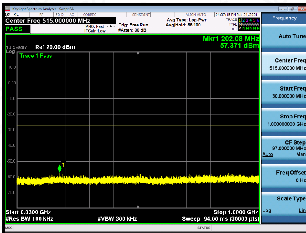
Test_Graph_802.11a_ANT1_5240_6Mbps_Frequency Band1
