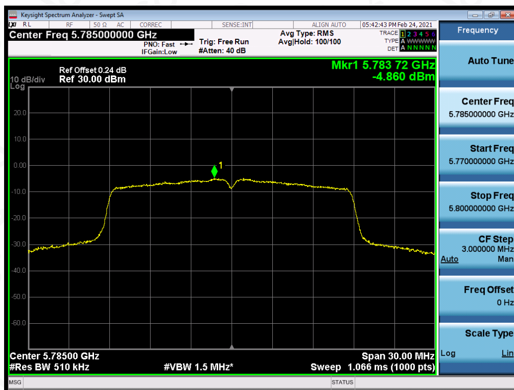
Test_Graph_802.11n20_ANT1_5785_MCS0_PSD
