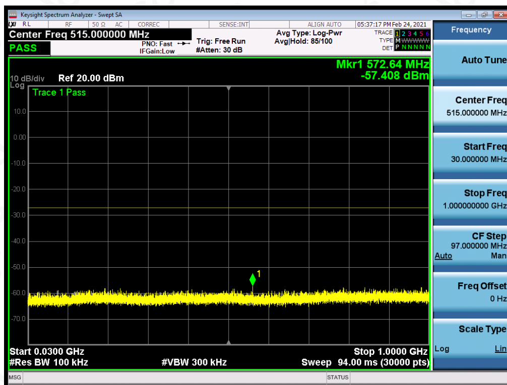
Test_Graph_802.11a_ANT1_5825_6Mbps_Frequency Band1
