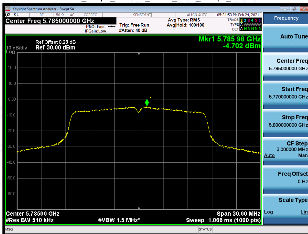
Test_Graph_802.11a_ANT1_5785_6Mbps_PSD
