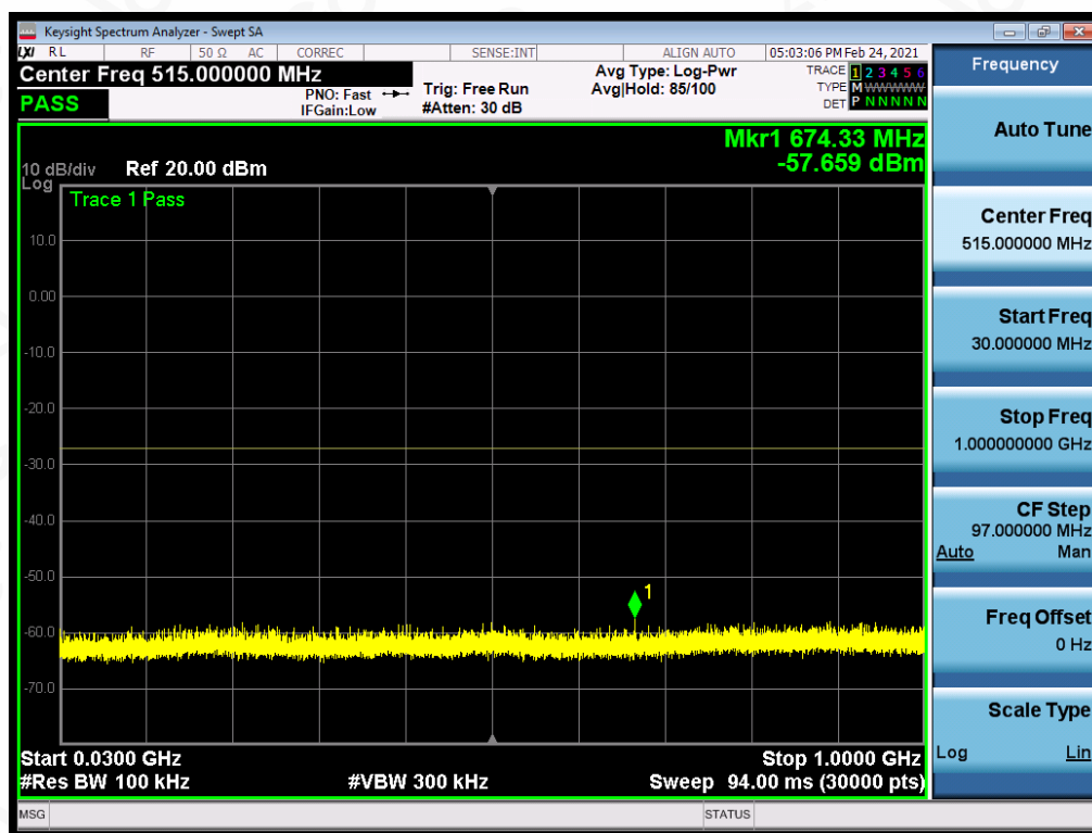
Test_Graph_802.11n40_ANT1_5190_MCS0_Frequency Band1
