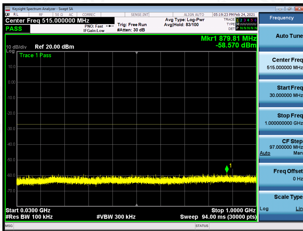
Test_Graph_802.11n40_ANT1_5230_MCS0_Frequency Band1
