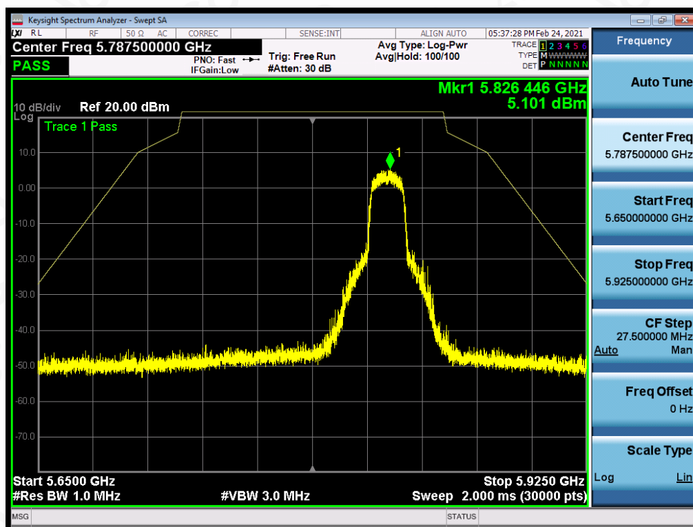
Test_Graph_802.11a_ANT1_5825_6Mbps_Frequency Band3
