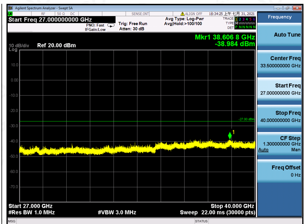
Test Graph 802.11a ANT1 5180 6Mbps Frequency Band 5
