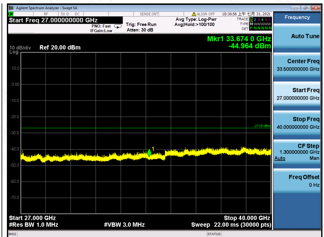
Test_Graph_802.11n40_ANT1_5755_MCS0_Frequency Band5
