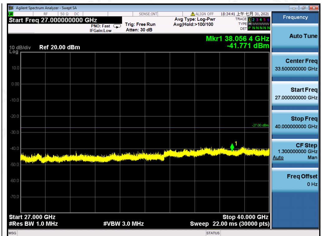
Test_Graph_802.11n40_ANT1_5190_MCS0_Frequency Band 5
