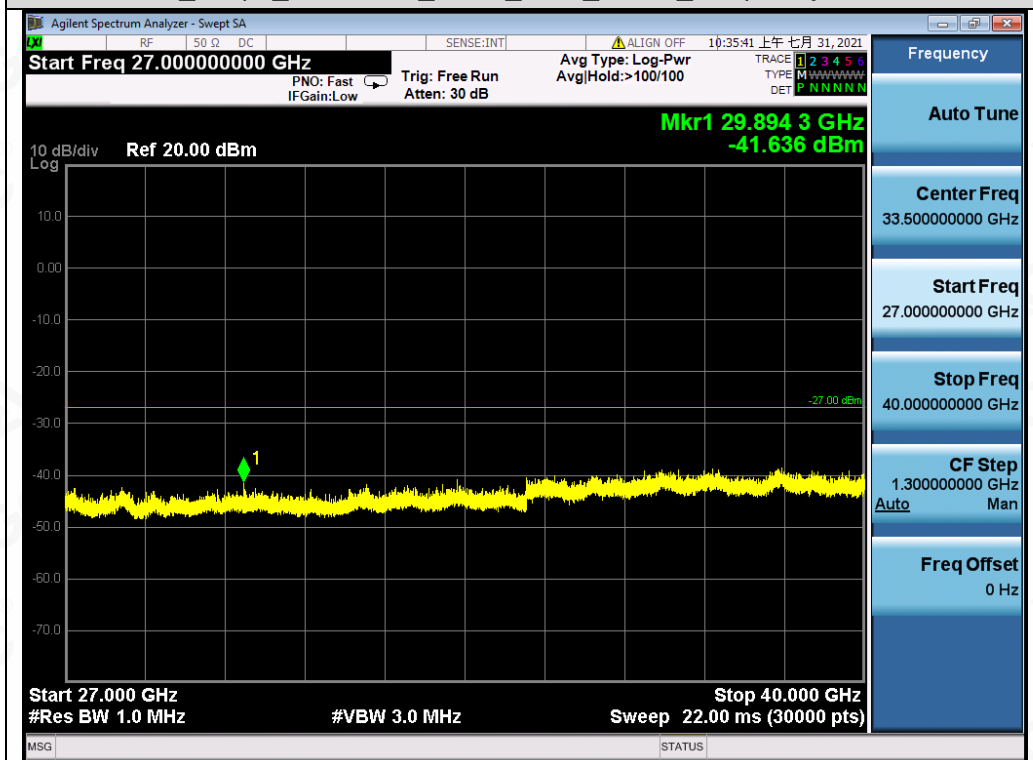
Test_Graph_802.11n40_ANT1_5310_MCS0_Frequency Band 5
