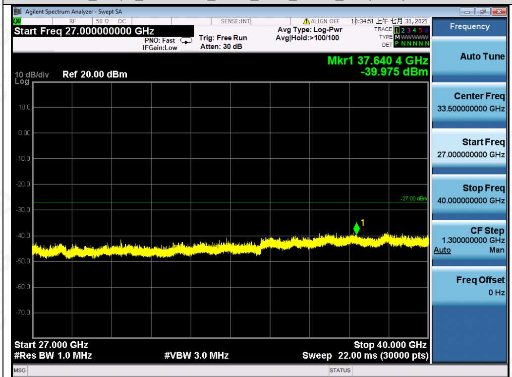
Test_Graph_802.11n40_ANT1_5230_MCS0_Frequency Band 5
