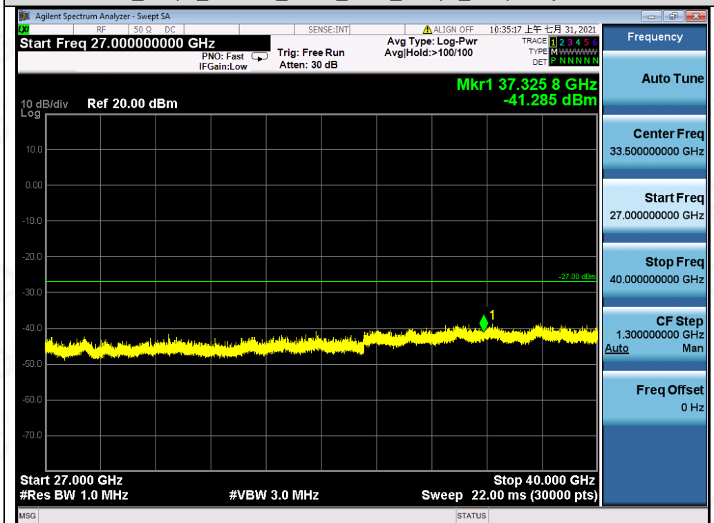
Test_Graph_802.11a_ANT1_5320_6Mbps_Frequency Band 5
