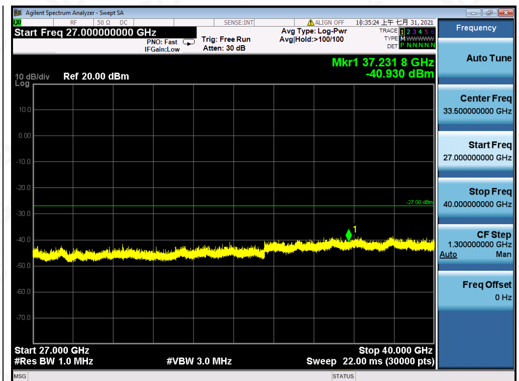
Test_Graph_802.11n40_ANT1_5270_MCS0_Frequency Band 5
