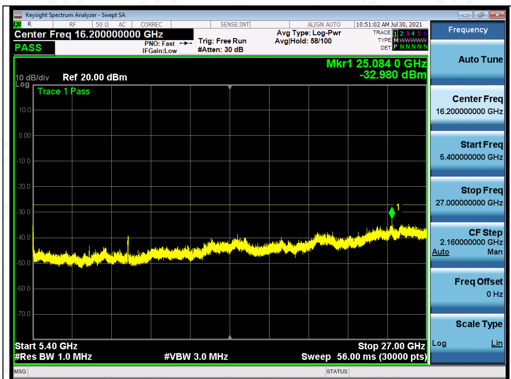
Test_Graph_802.11n40_ANT1_5310_MCS0_Frequency Band 4
