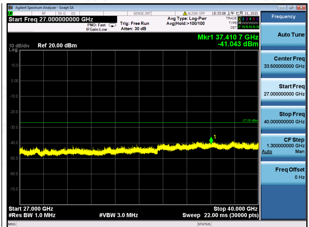
Test_Graph_802.11a_ANT1_5260_6Mbps_Frequency Band 5
