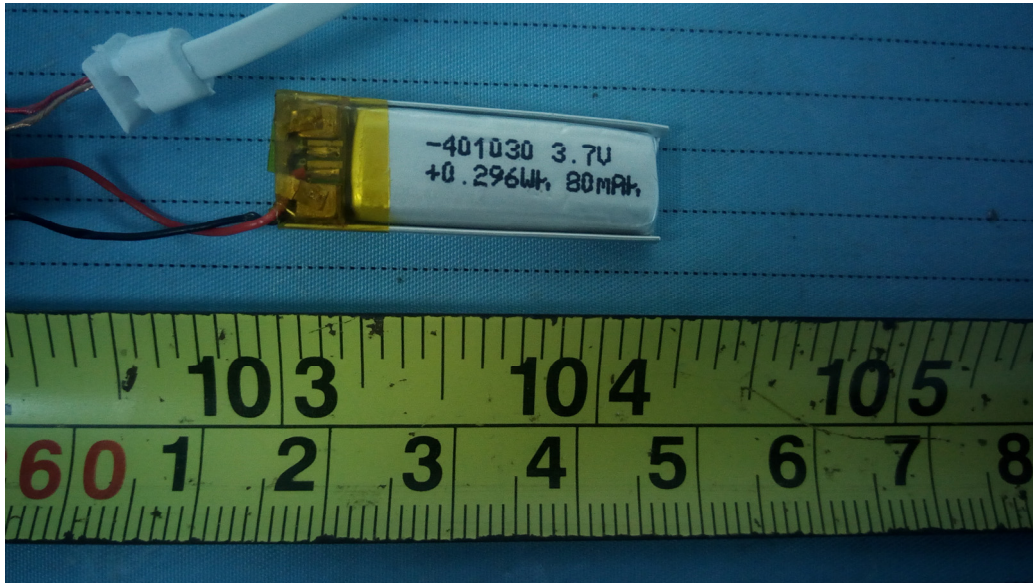
EUT – Battery Top View
