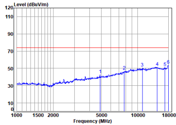
11n_40M_TX_CH_09_Vertical-Peak
