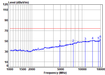
11n_40M_TX_CH_09_Horizontal-Peak
