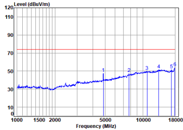
11n_40M_TX_CH_03_Horizontal-Peak
