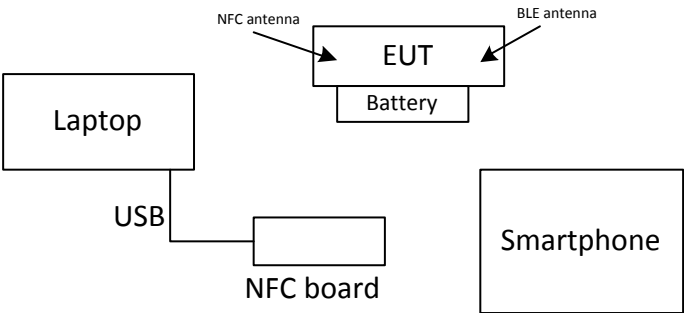
Figure 3.6-1: Setup diagram
