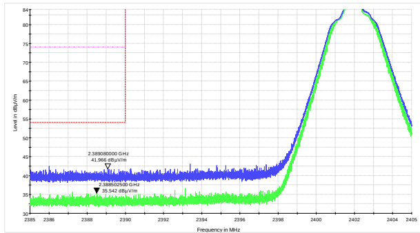
Figure 8.3-6: Lower band edge emission within restricted bands at 2.4 GHz
