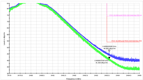
Figure 8.3-7: Upper band edge emission within restricted bands at 2.4835 GHz
